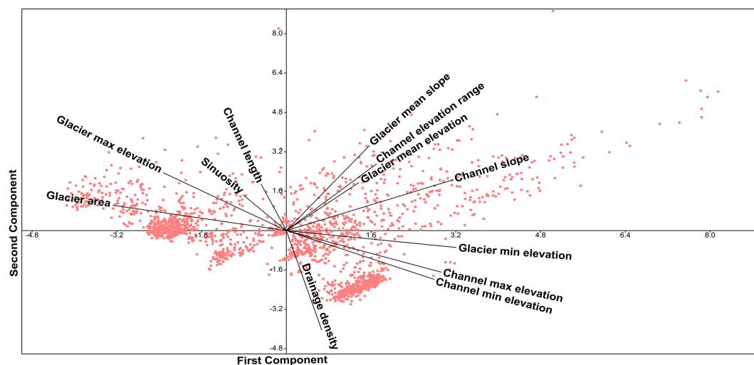
Figure A2. A biplot from a PCA analysis showing Principal Components 1 and 2, which were used for visually identifying clusters and overlaid with a loading plot (see Fig. A1).
