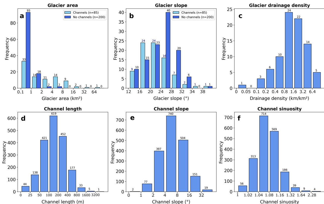
Figure 3. Histograms of extracted metrics. Note that the x axis uses a log scale (except for panel b ) and the numbers above each bar represent the number of channels/glaciers within each class. The range shown by each bar is indicated by the x axis values to either side. The range is exclusive of the lower value and inclusive of the higher one (e.g., > 1 \leq 2 ). ( a ) Glacier area (km 2 ); ( b ) glacier slope (°); ( c ) glacier drainage density (km km -2 ); ( d ) channel segment length (m); ( e ) channel slope (°); and ( f ) channel sinuosity.
