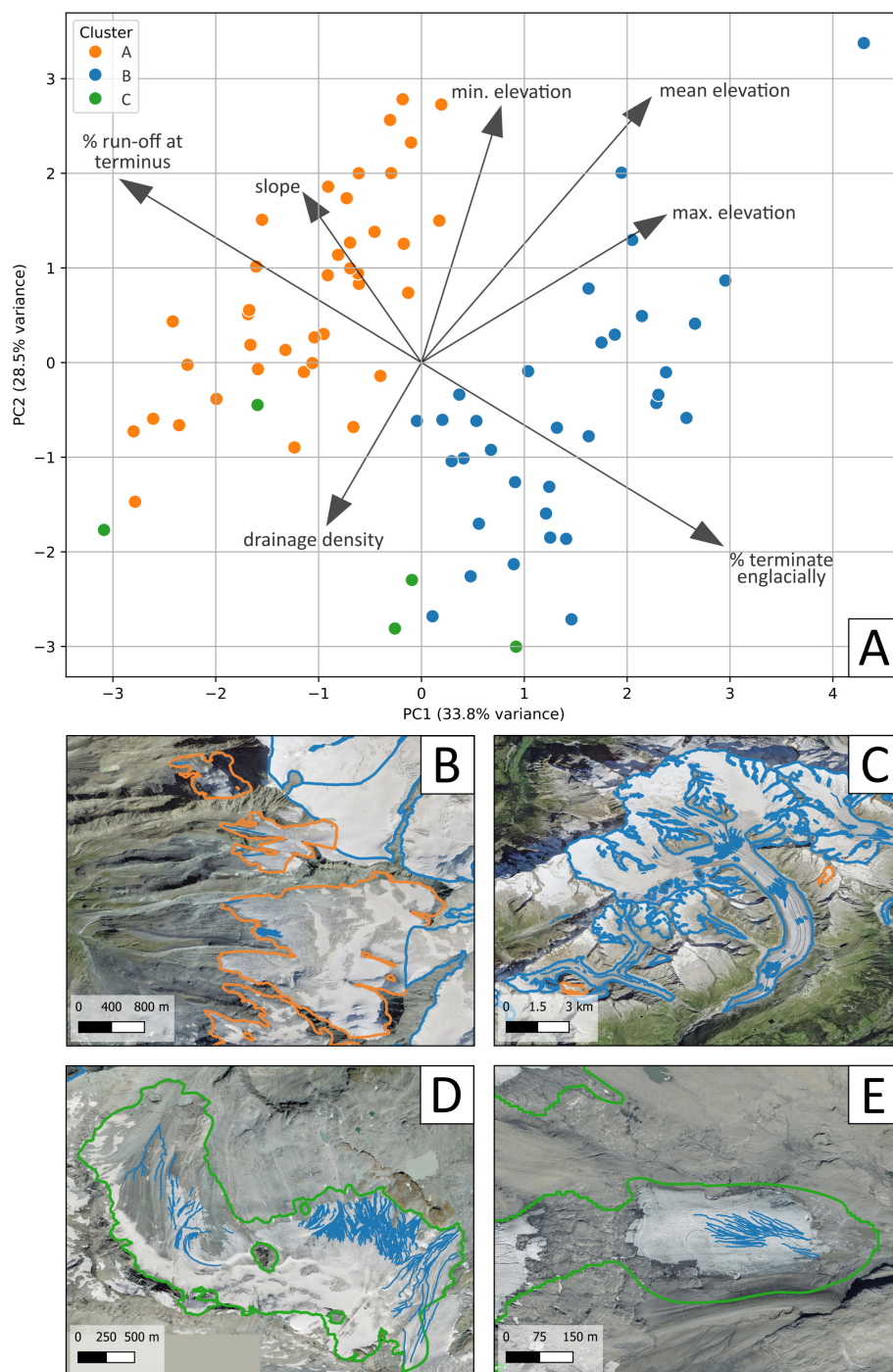
Figure 7. Glacier types across Valais categorised according to their terminus locations and characteristics. (A) A principal component analysis biplot of glacier characteristics overlaid with a loading plot. Each point is coloured based on its respective cluster (B). A group of type A glaciers, the largest being Mellichgletscher (centre right). (C) Several type B glaciers, e.g., Grosser Aletschgletscher (center right) and Oberaletschgletscher (far left). (D) An example of a Type C glacier – the Oberer Theodulgletscher. (E) A disconnection that has occurred from the main part of Wildstrubelgletscher. Both parts of the glacier are still treated as one connected mass based on the glacier outlines used, and are classified as Type C.
