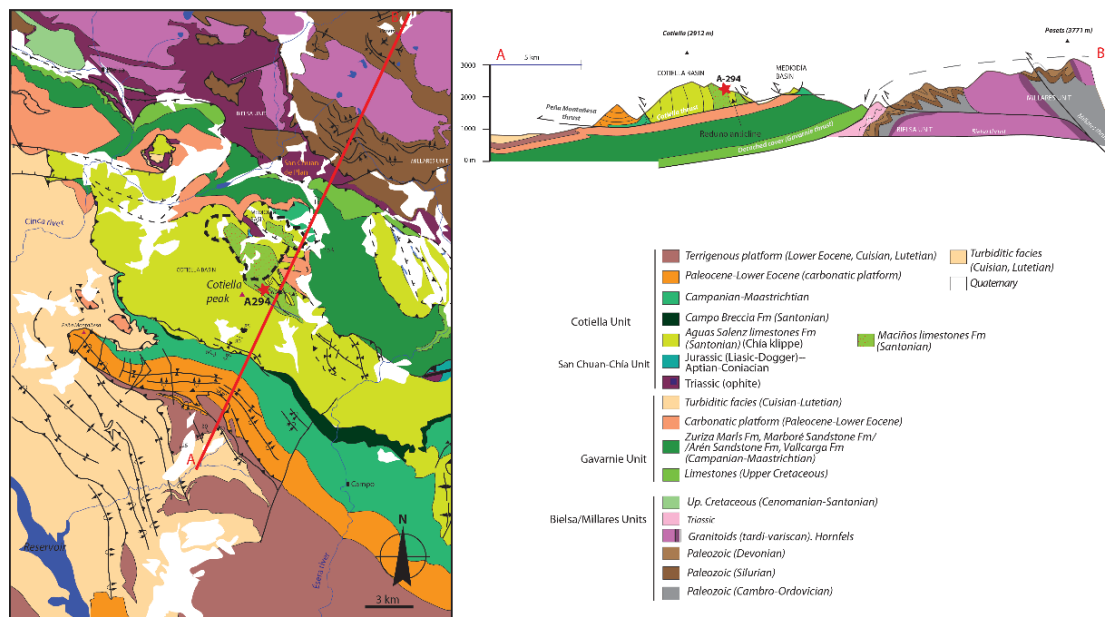
Figure S1: Simplified geological map of the Cotiella area based on IGME Bielsa (179) Ríos et al., (1982) and Campo (212) Robadoret al., (1999) and López-Mir et al., (2015), and cross-section (red line on the map). Red star in the cross-section indicates the location of the A294 ice cave.
