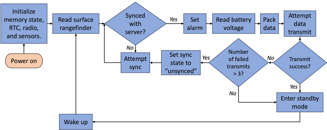
Figure 4. Node flow diagram. The high-level logic of a SnoTATOS node equipped with only a snow surface rangefinder is shown. Additional sensors may be added, which would be read at the same stage as the surface rangefinder.
