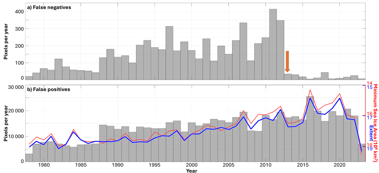
Figure 3. (a) False negatives and (b) false positives for each year, in number of pixels. Note the different y axes. The orange arrow on (a) highlights the beginning of reliable sea ice thickness observations, and therefore the effect of merging the SIC and SIT labelled datasets. The red and blue lines on (b) are the minimum sea ice area and extent, respectively (winter months only), flipped vertically to highlight the correlation. Note that the 2023 data stop in April, hence the higher sea ice areas and extents.
