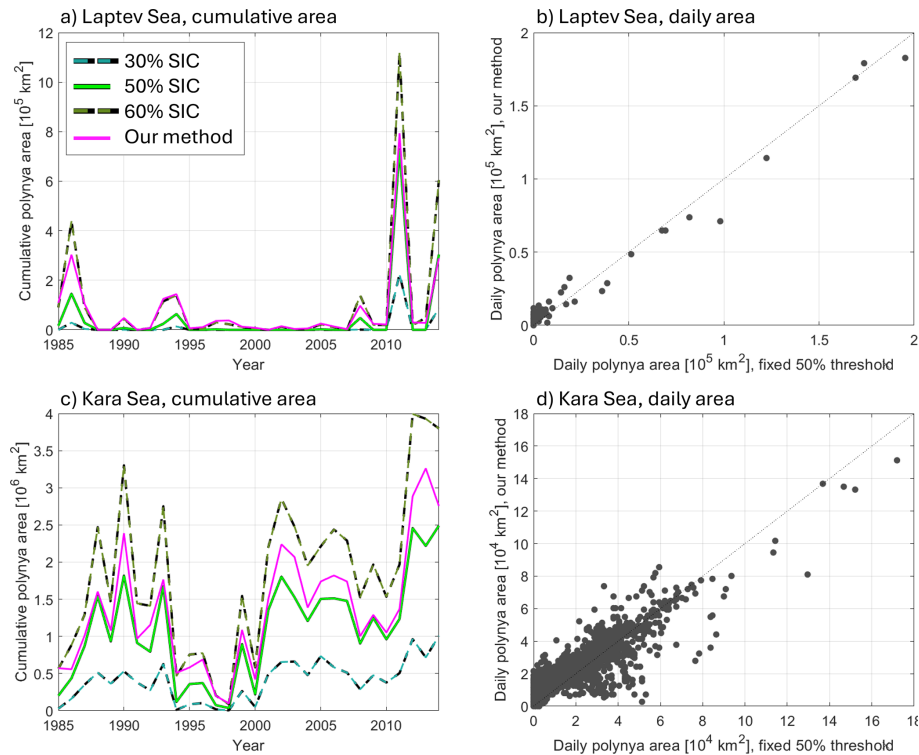
Figure 8. Polynyas in the Laptev (a, b) and Kara seas (c, d) in MIROC6 daily data. (a, c) Comparison of the cumulative winter polynya area retrieved by our method (magenta) and several commonly used fixed sea ice concentration thresholds (green). (b, d) Comparison of all the daily polynya areas between our method and the 50 % threshold it was trained on; black line is the x = y unit line.
