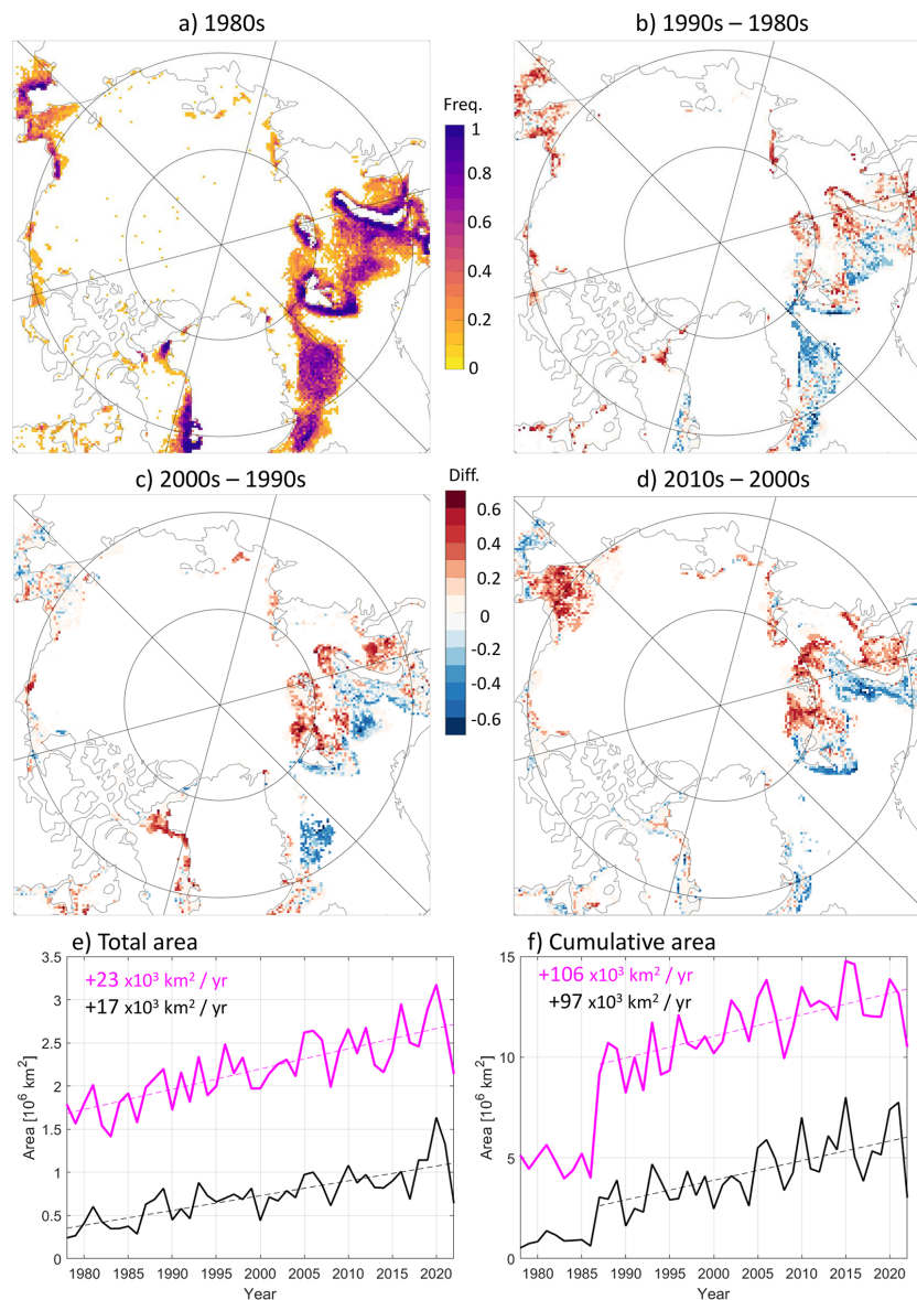
Figure 6. Variability exhibited by our results: Combining our true and false positives, for each pixel (a) frequency in polynya opening in the 1980s, i.e. out of the 10 winters of that decade, how many had a polynya (only > 0 shown); (b–d) difference in polynya opening between two consecutive decades; (e) total and (f) cumulative polynya area of each winter in our results (magenta) and in Wong et al. (2025) (black) for the entire Arctic, along with the corresponding linear trends. See text for definition of each area.
