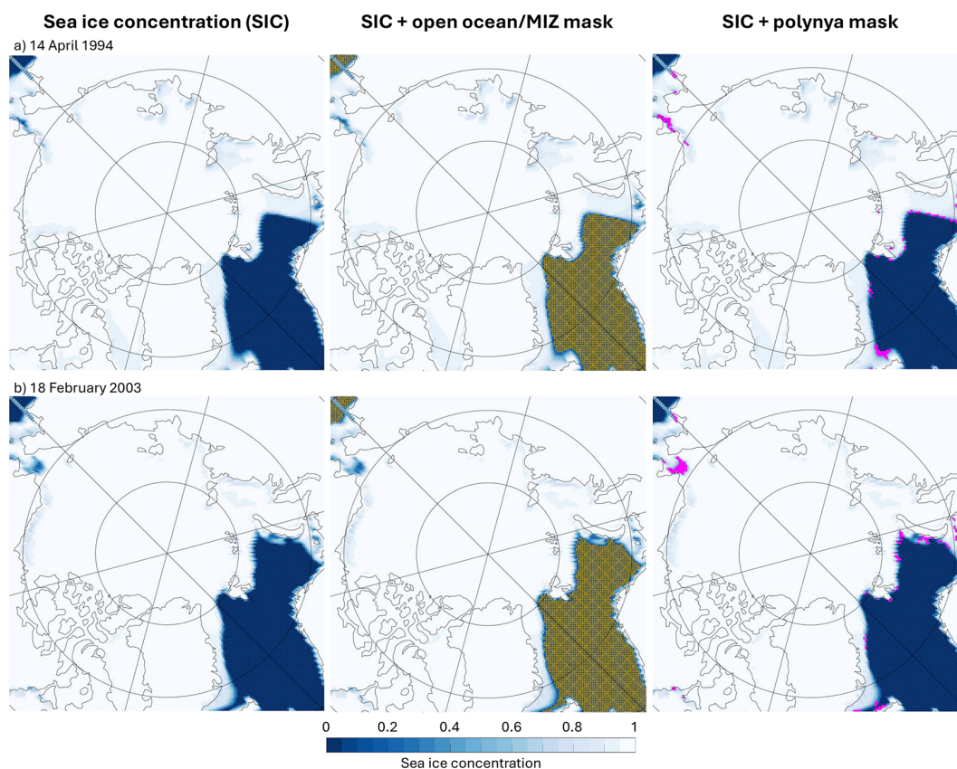
Figure 7. Two example results, on (a) 14 April 1994 (top) and (b) 18 February 2003 (bottom), of the model MIROC6's daily sea ice concentration data (left), with superimposed the resulting GMM-produced open ocean/MIZ mask (middle, orange asterisks) or the polynya mask (right, magenta).
