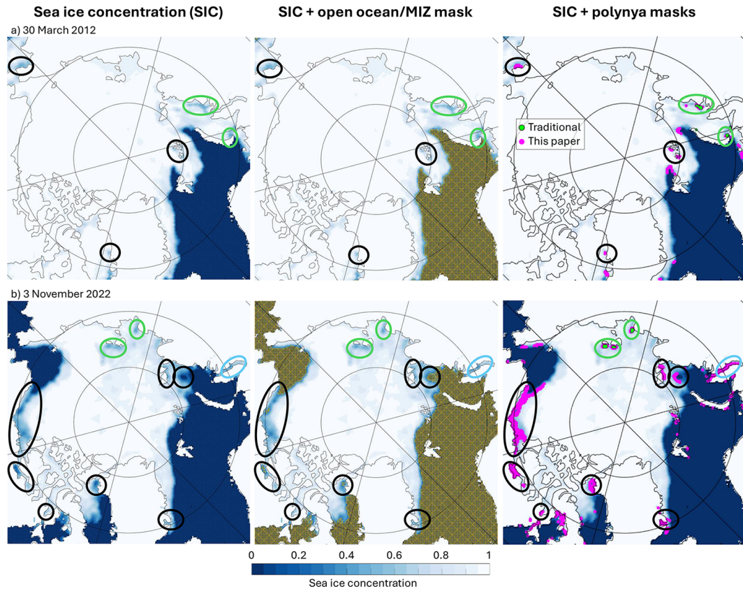
Figure 5. Two example results, on (a) 30 March 2012 (top) and (b) 3 November 2022 (bottom), of the original daily sea ice concentration data (left), with superimposed the resulting GMM-produced open ocean/MIZ mask (middle, orange asterisks) or the polynya masks (right, green and magenta). Green dots are the polynyas detected with a traditional threshold method, i.e. the labelled dataset we used for training, and magenta dots are the polynyas detected with our method. Green circles highlight areas where the two methods agree. Black circles highlight areas with false positives that we argue are correct, while the blue circle on (b) is a special case, see text.
