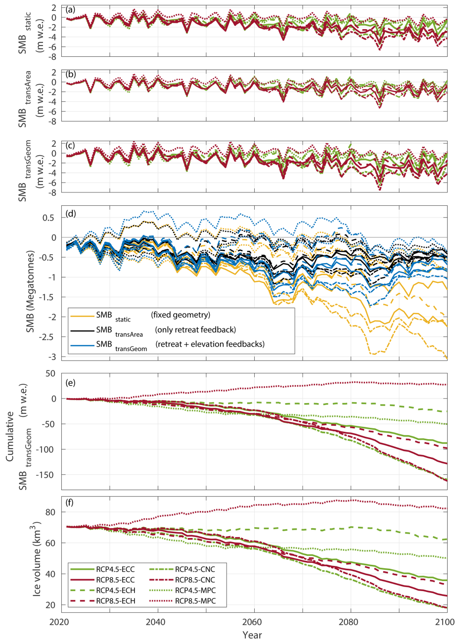
Figure 11. Future evolution of SMB and ice volume 2021–2100 across the ensemble of climate model forcings, cf. Table 2. (a) SMB with fixed present-day ice geometry (SMB static ); (b) SMB over the modelled area evolving over time, without accounting for the SMB-elevation feedback (SMB transArea ; see Sect. 4.3); (c) SMB over a transiently updated area and elevation, (SMB transGeom ); (d) total SMB of the representations in (a) – (c) in Megatonnes ( 10^6 \text{ m}^3 \text{ w.e.} ), using a 5-year moving mean; (e) Cumulative SMB transGeom ; (f) Modelled ice volume with SMB transGeom . Line styles shown in the legend in (f) are consistent in (a) – (c) and (e) – (f) , representing climate model combinations ECEARTH/CCLM (ECC), ECEARTH/HIRHAM (ECH), CNRM/CCLM (CNC), and MPI/CCLM (MPC).
