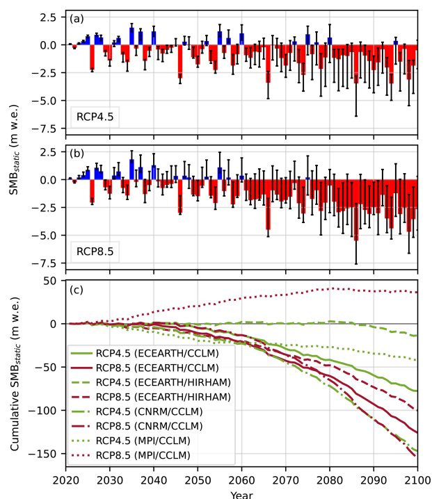
Figure 4. Modelled glacier-wide annual reference surface mass balance ( SMB_{static} , fixed DTM 2020 geometry and 2019 area) for Jostedalsbreen over the period 2021–2100. Results are presented as median annual mass balance across climate model combinations for (a) RCP4.5 and (b) RCP8.5, and (c) cumulative mass balance for each model and RCP combination. Bars in (a) and (b) show median modelled mass balance and whiskers show spread of models (minimum and maximum values).
