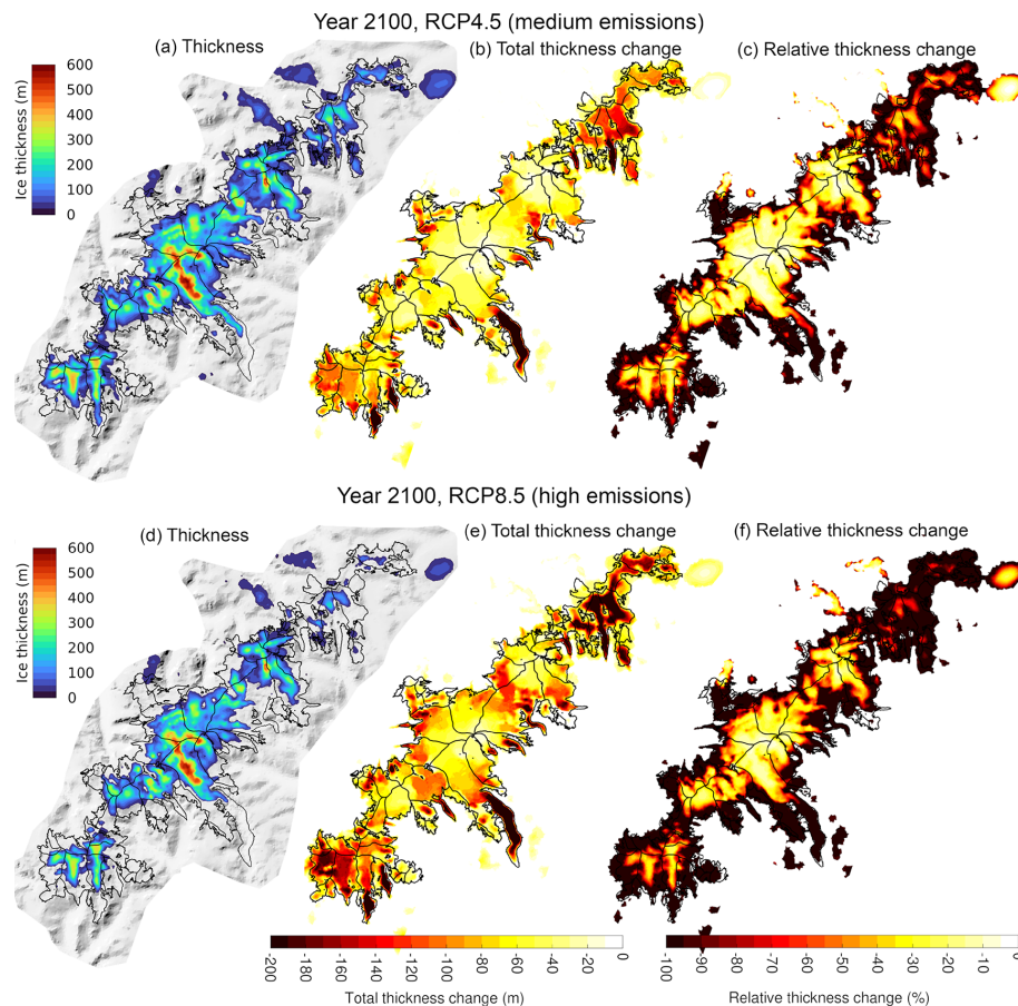
Figure 6. Future model thickness and thickness change under medium (a–c) and high (d–f) emissions, using ECEARTH/CCLM climate forcing. (a, d) Modelled ice thickness in year 2100; (b, e) Total ice thickness change (future–present); (c, f) Relative thickness change. In (e)–(f), yellows means a slight surface lowering, while dark red implies strong thinning. In (c) and (f), −100 % thickness change means complete deglaciation
