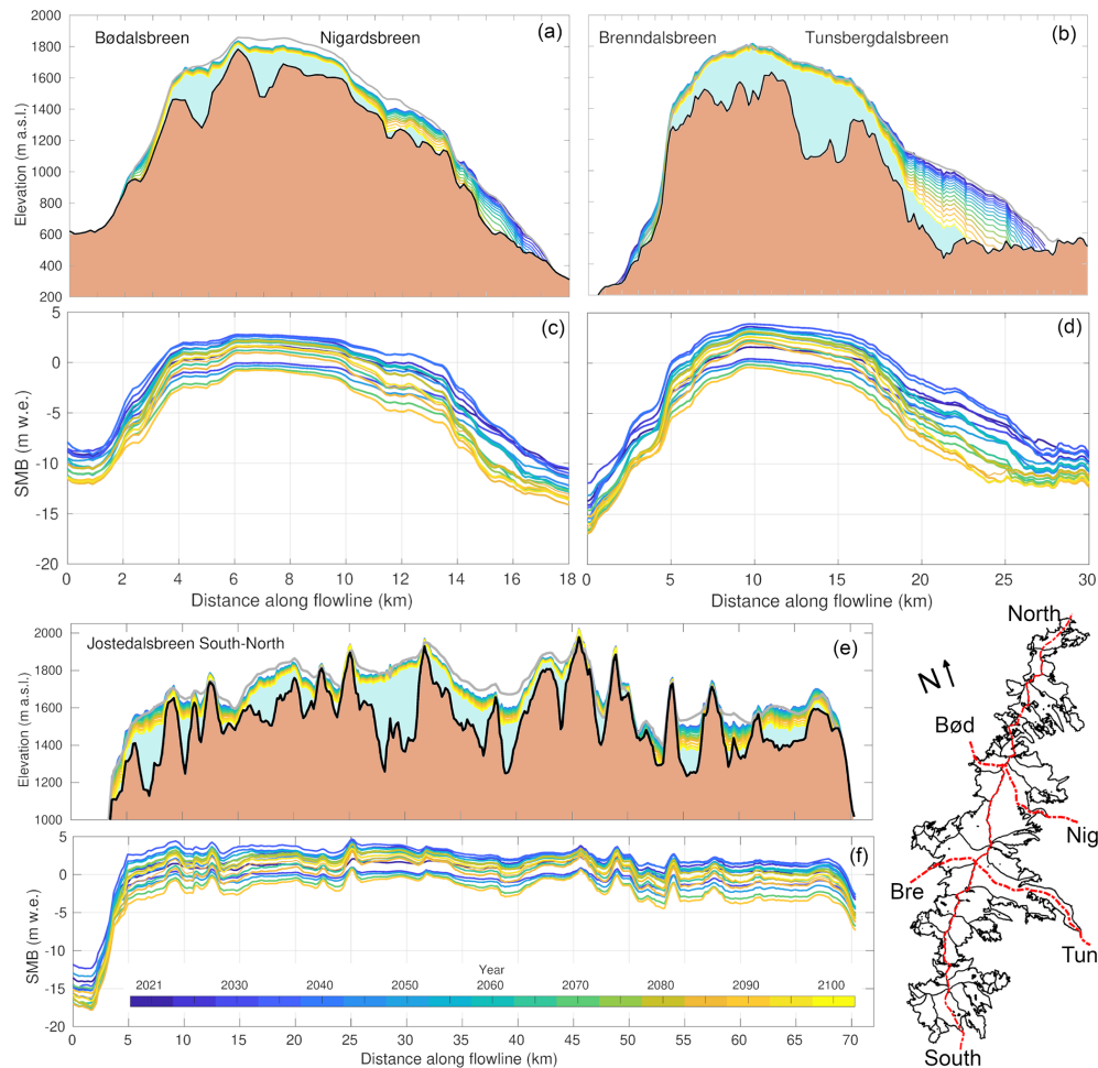
Figure 7. Elevation of bedrock and modelled ice-surface evolution (a, b, e) and SMB evolution (c, d, f) 2021–2100 under RCP4.5 (ECEARTH/CCLM) for three transects on Jostedalsbreen. Panels (a), (b) and (e) illustrate a consistent, progressive glacier surface lowering over time, despite some decadal variability in surface mass balance (c, d, f). The three transects are shown in the inset map, which is slightly rotated for visibility.
