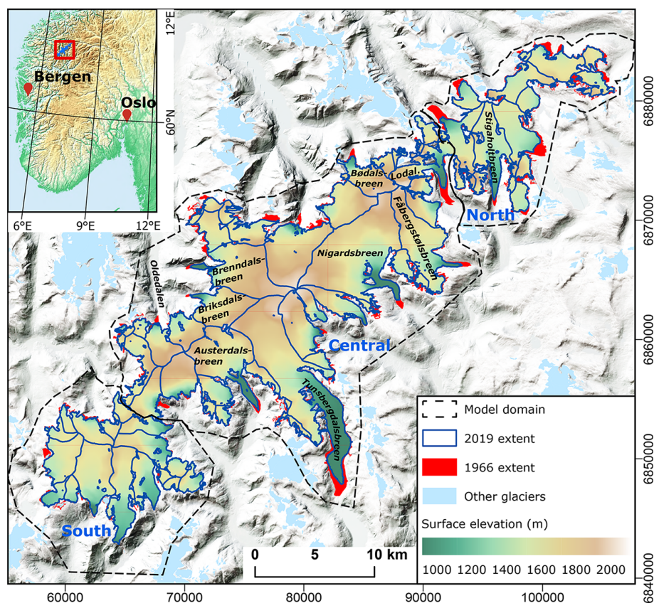
Figure 1. Ice-surface topography of Jostedalsbreen ice cap. Key outlet glaciers are named. Observed ice-cap extents in 1966 and 2019 are shown (Andreassen et al., 2023), as well as individual glacier catchments (blue). The inset map shows the location of Jostedalsbreen in southern Norway. Coordinates in UTM 33N, datum ETRS89 on main map and in geographical coordinates on inset.
