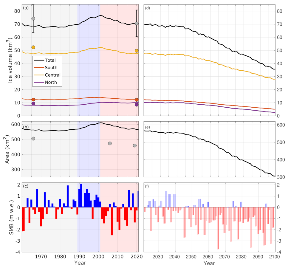
Figure 2. Simulated historical change (a–c) and future (d–f) evolution with experiment Future4.5-ECC (cf. Table 2). Recent historical periods of little change (gray), ice-cap growth (blue) and decay (red) are shaded in (a)–(c). Observed volumes and areas are shown as filled circles in (a) and (b). In (c), historical SMB with evolving model area is shown ( \text{SMB}_{\text{transArea}} ), but without elevation changes, since these make little difference (Sect. 5.2). Shown in (f) is SMB with transiently evolving geometry ( \text{SMB}_{\text{transGeom}} ), including the SMB–elevation feedback and area changes.
