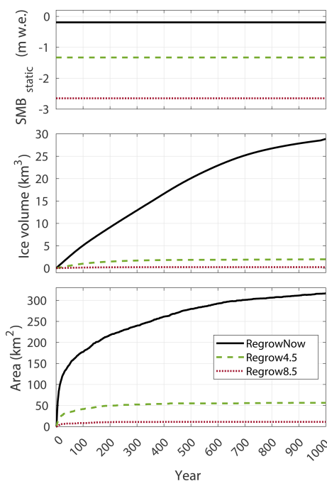
Figure A3. Model evolution of (a) SMB_{static} , (b) ice volume, and (c) area in experiments aiming to grow Jostedalsbreen from ice-free conditions. See Table 2 for experiment details.
