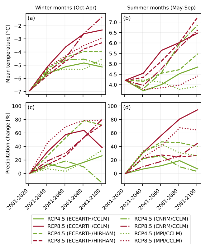
Figure A5. Future changes in (a) and (b) mean temperature and (c, d) total precipitation in (a) and (c) winter (October–April) and (b, d) summer (May–September) months for the ensemble of climate model forcing.
