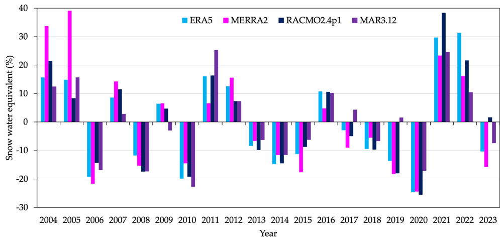
Figure 5. Yearly snow water equivalent anomaly (2004–2023 climatology, in %).
