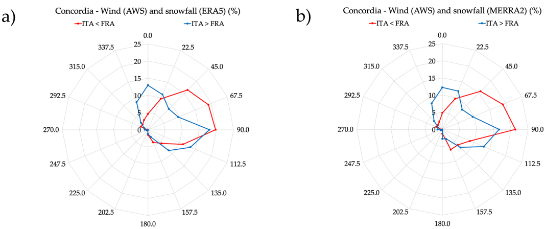
Figure 12. Direction of the wind near Concordia Station during snowfall events; the “ITA < FRA” and “ITA > FRA” cases are considered (see the text for the details). Wind data taken from the Italian AWS of Concordia and snowfall from (a) ERA5 and (b) MERRA2.
