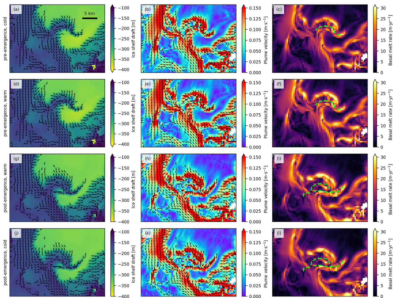
Figure A5. (a–c) Ice shelf draft, LADDIE plume velocity, and LADDIE basal melt rate of the pre-emergence experiment. (d–f) same as (a)–(c) but using ocean forcing from the warmer post-emergence experiment. (g–i) Ice shelf draft, LADDIE plume velocity, and LADDIE basal melt rate of the post-emergence experiment. (j–l) same as (g)–(i) but using ocean forcing from the colder pre-emergence experiment.
