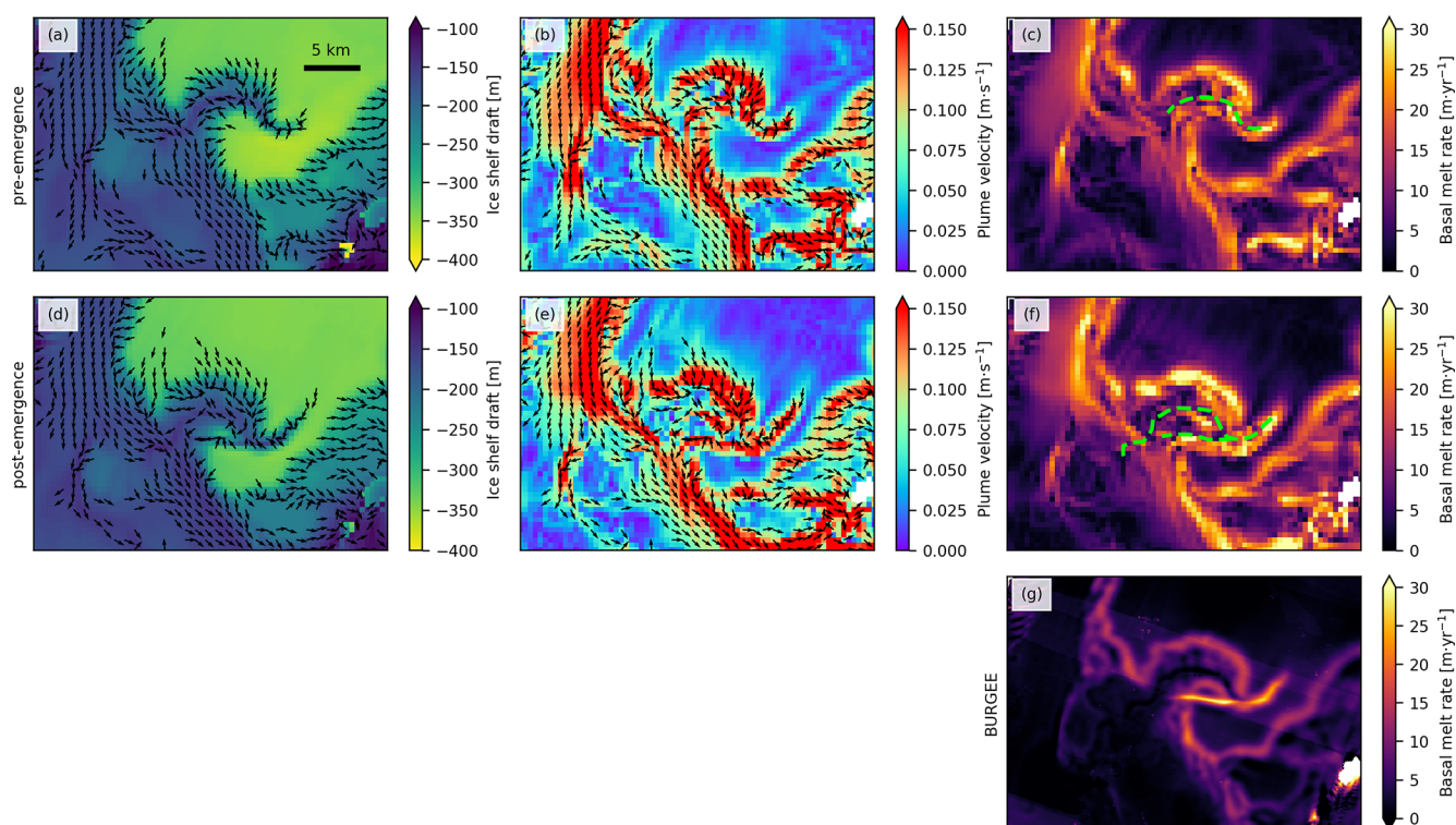
Figure 8. (a–c) Ice shelf draft, LADDIE plume velocity, and LADDIE basal melt rate of the pre-emergence experiment. (d)–(f) Same as (a)–(c) but for the post-emergence experiment. Arrows on (a)–(b) and (d)–(e) are the plume velocities. The dashed green line in (c) marks the location of the original channel in 2012/2013 and the dashed green line (f) marks the location of the new channel in 2021/2022. (g) BURGE basal melt rates.
