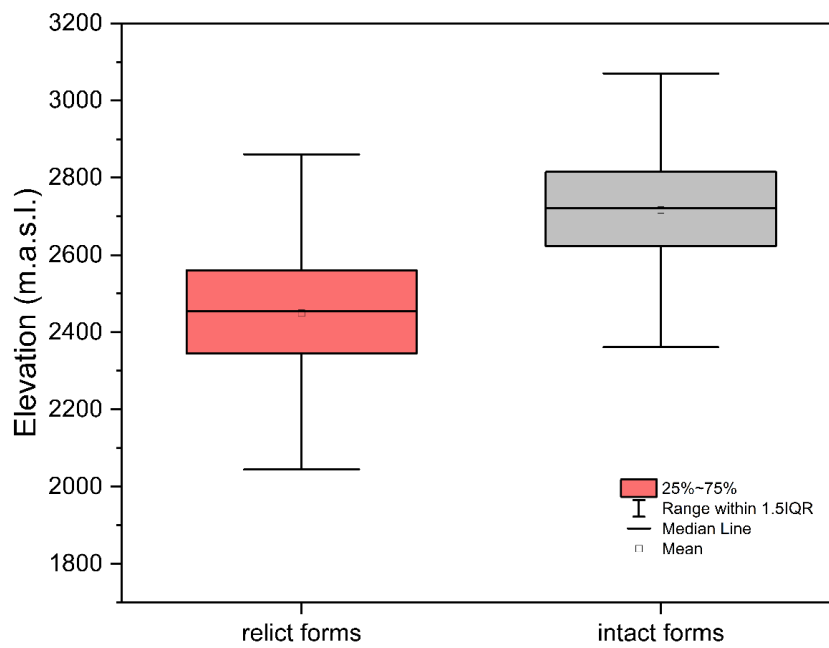
Figure S1. Altitude value distributions in the periglacial features mapped in the study area (geomorphological classification according to Scotti et al., 2013).
