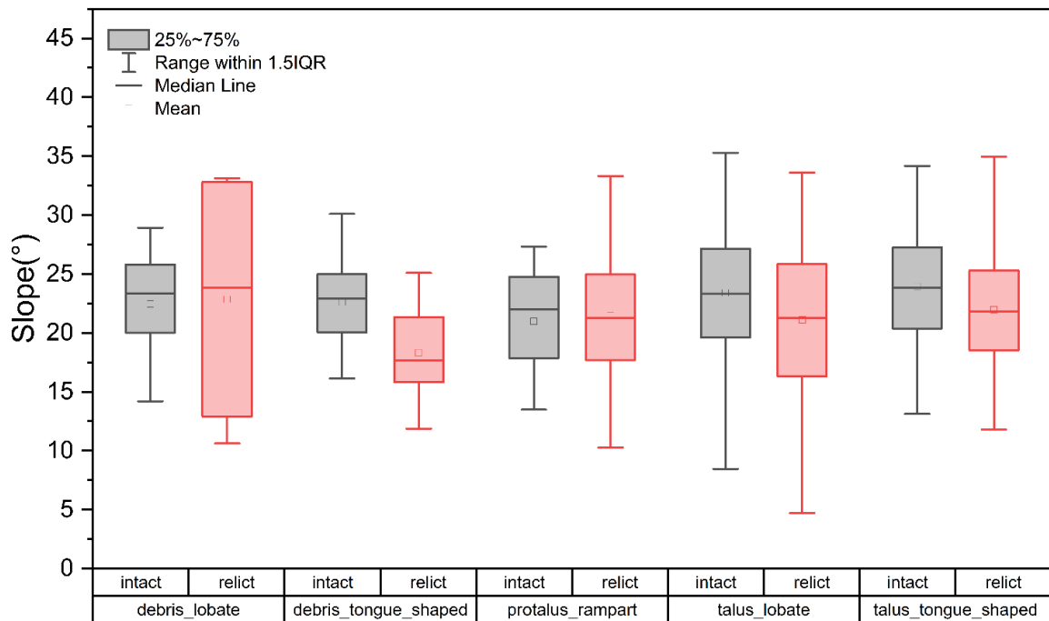
Figure S2. Topographic slope distributions in the periglacial features mapped in the study area (geomorphological classification according to Scotti et al., 2013).
