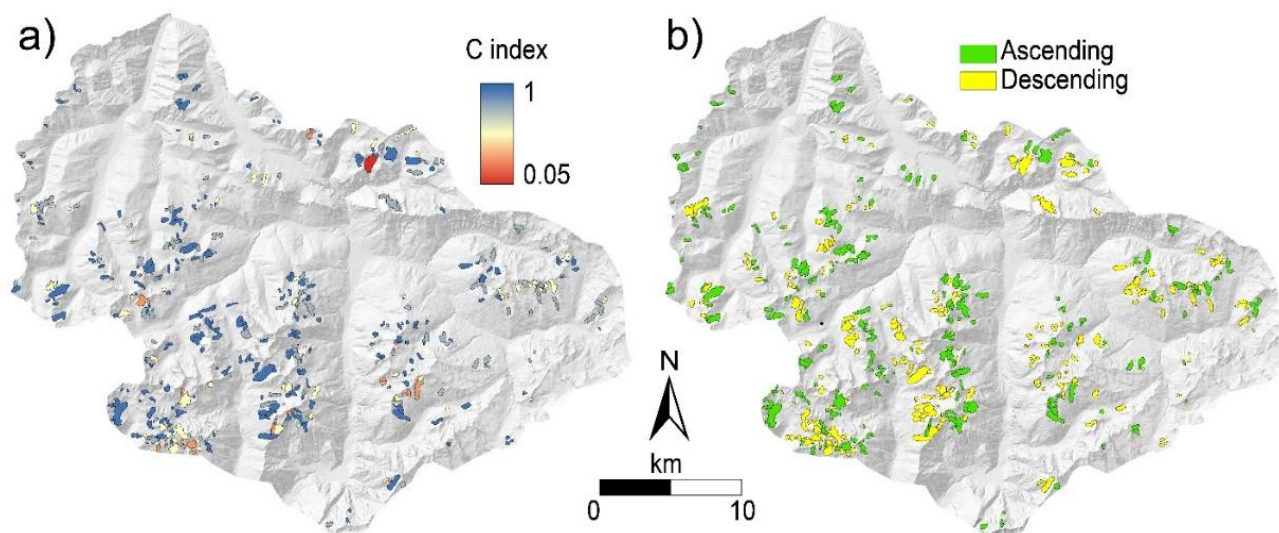
Figure S4. Maps portraying: a) the visibility of each periglacial landform to SAR sensors. Favourably oriented slopes have higher C index; b) most suitable satellite geometry for each mapped periglacial landform.
