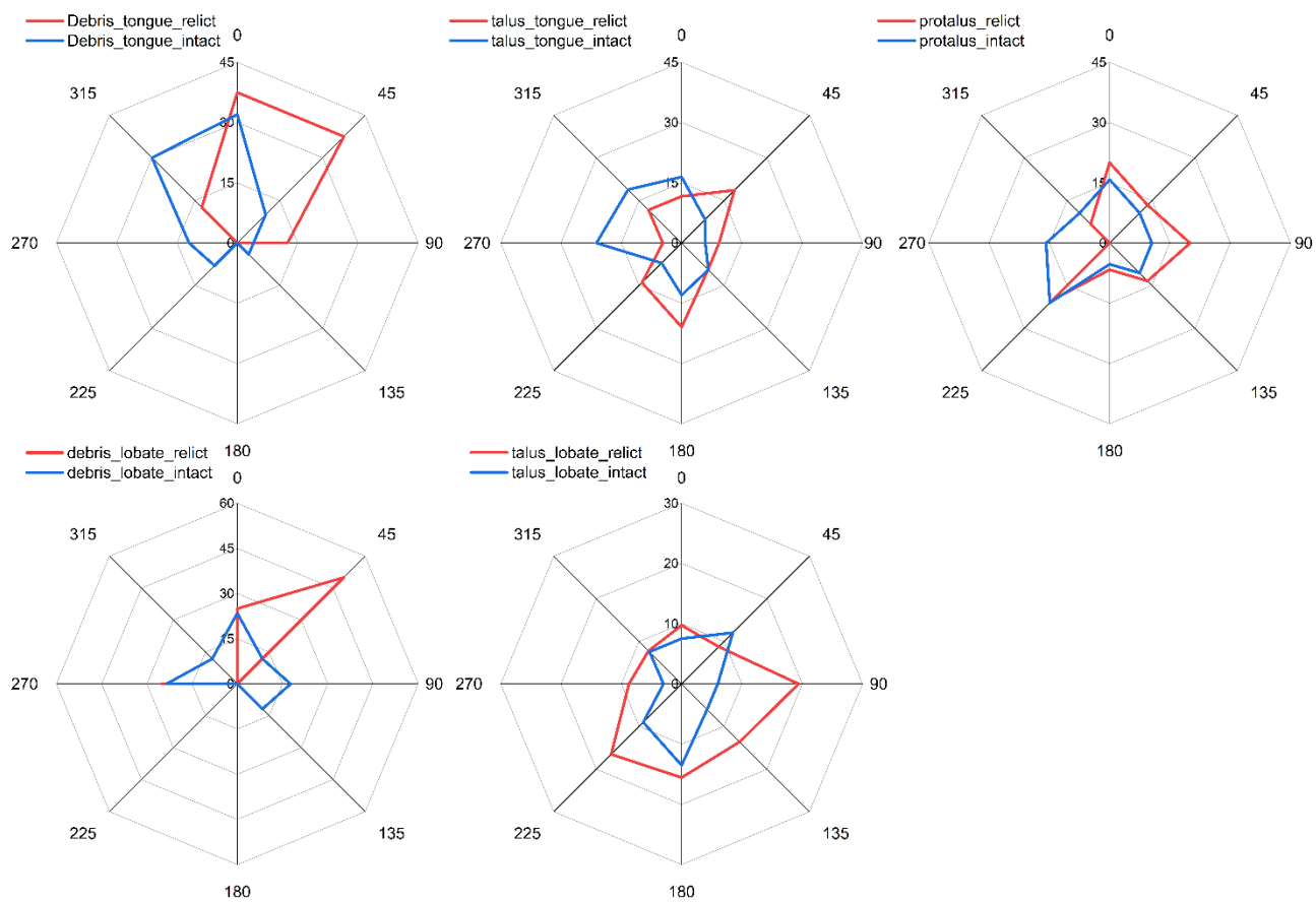
Figure S3. Topographic aspect distributions in the periglacial features mapped in the study area (geomorphological classification according to Scotti et al., 2013).
