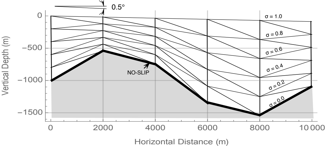
ISMIP-HOM Test Problem B - No Slip
