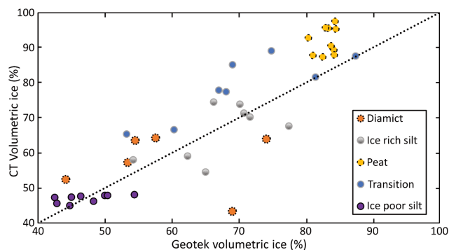
Figure 17. Estimated volumetric ice contents from CT image processing vs. calculated values from the MSCL method.
