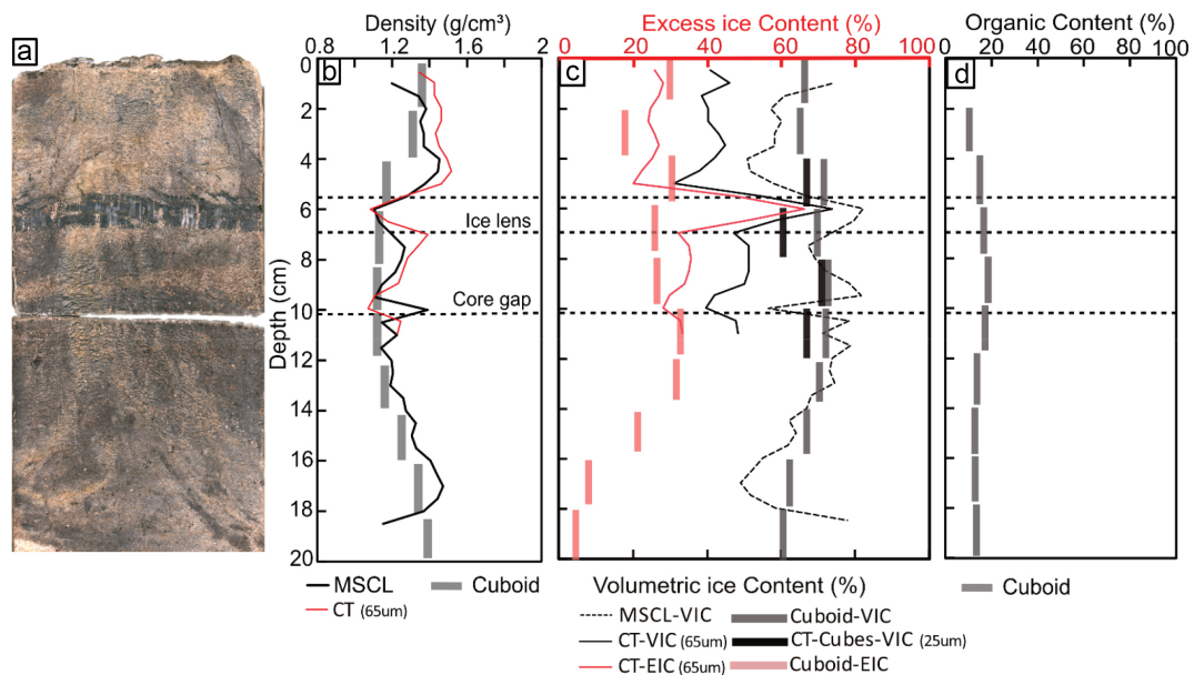
Figure 6. (a) MSCL image of the ice-rich and organic-rich silt core, (b) bulk density, (c) ice contents, and (d) organic content distribution in core depth.
