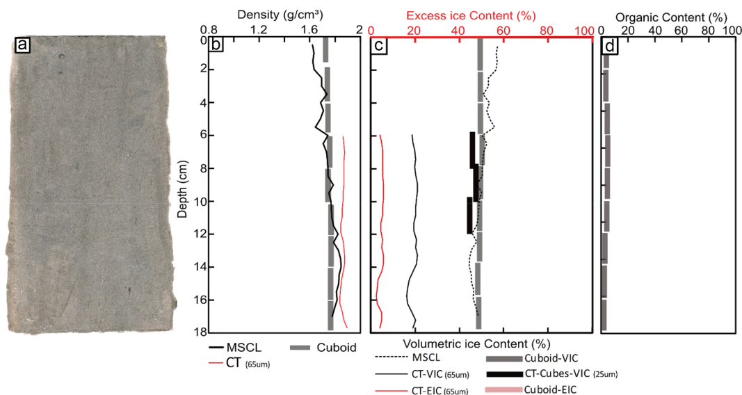
Figure 9. (a) MSCL image of the ice-poor silt core, (b) bulk density, (c) ice contents, and (d) organic content distribution in core depth.
