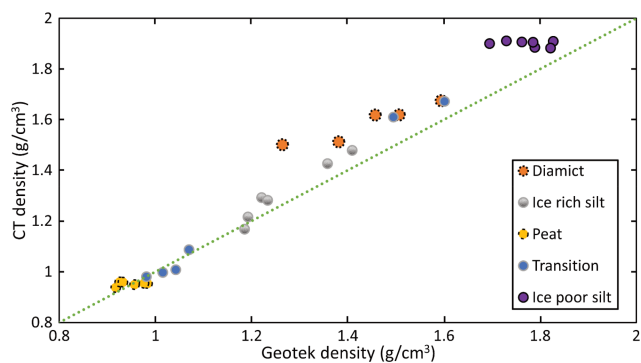
Figure 16. Estimated bulk density from CT image processing vs. calculated values from the MSCL method.
