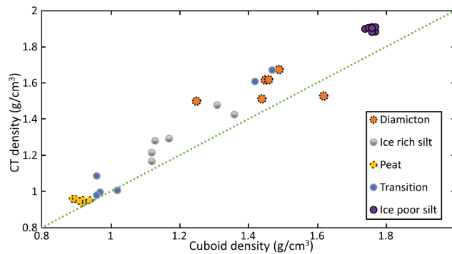
Figure 13. Estimated densities from CT image processing of 65 μm scans vs. calculated ones from the cuboid method.
