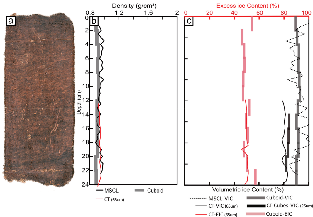
Figure 10. (a) MSCL image of the peat core, (b) bulk density, and (c) ice contents.
