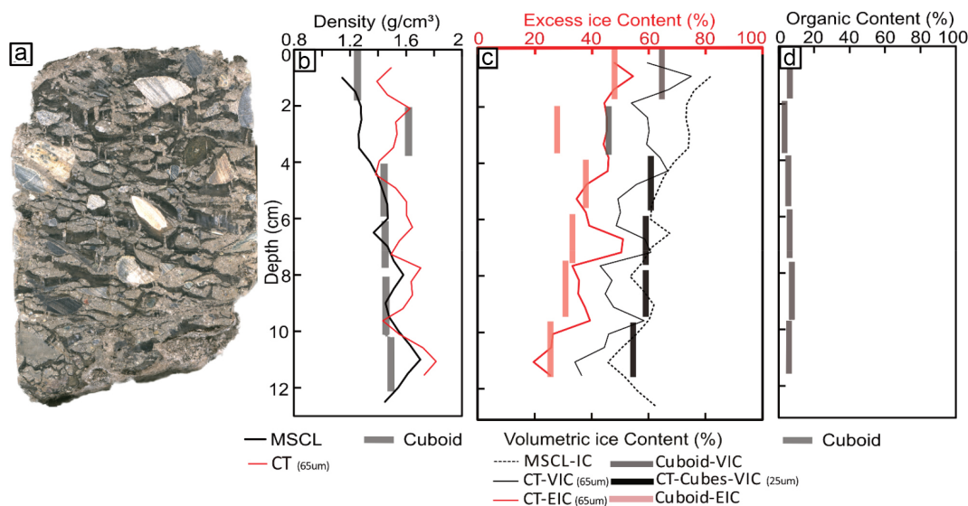
Figure 8. (a) MSCL image of the diamicton core, (b) bulk density, (c) ice contents, and (d) organic content distribution in core depth.
