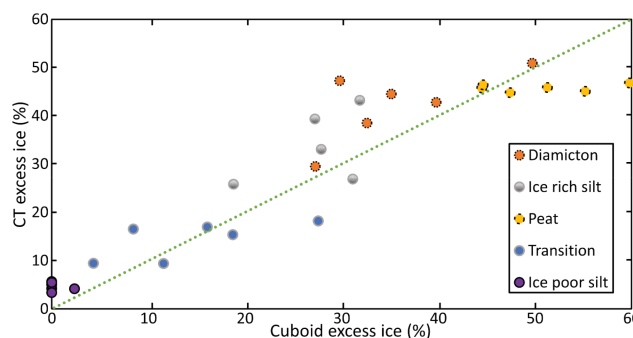
Figure 14. Estimated excess ice contents from CT image processing of 65 μm scans vs. calculated values from the cuboid method.
