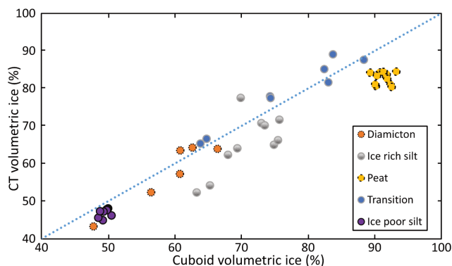
Figure 15. Estimated volumetric ice contents from CT image processing of 65 \mu\text{m} scans vs. calculated values from the cuboid method.
