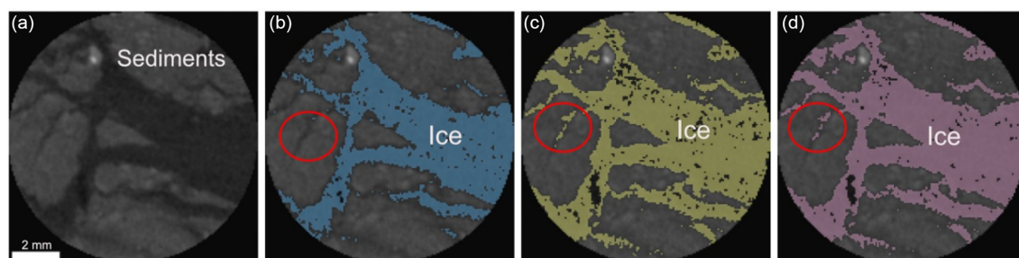
Figure 3. Overview of a slice from ice-rich silt core (a) before image processing, (b) after the first step, (c) after the second step, and (d) after the third step of image processing using the Otsu method.
