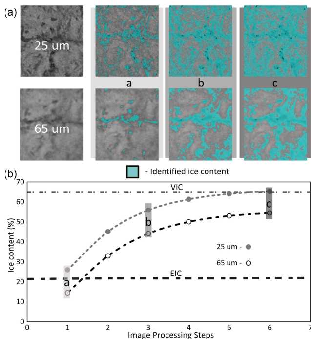
Figure 12. (a) CT ROIs taken from the 65 and 25 μm cube scans (BH12F-138-10-12 cm). (b) Identified ice contents at each image processing step using the Otsu split method.
