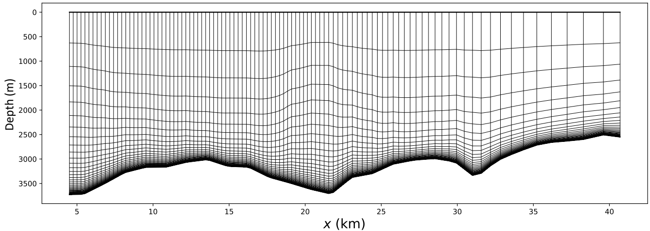
Figure S1. Grid used in the forward model which is regular in the forward model coordinate system, but is shown here in the physical coordinate system (x, \text{Depth}) . This figure is for illustrative purposes only, the grid used in the final forward model has 600 nodes in the x direction, more than are shown here.
