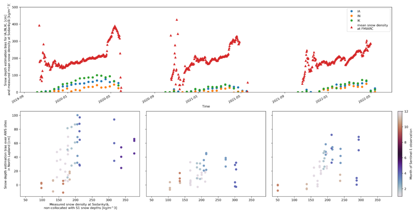
1 Figure S1: Bias evolution of the snow depth as a function of the days of the year.
