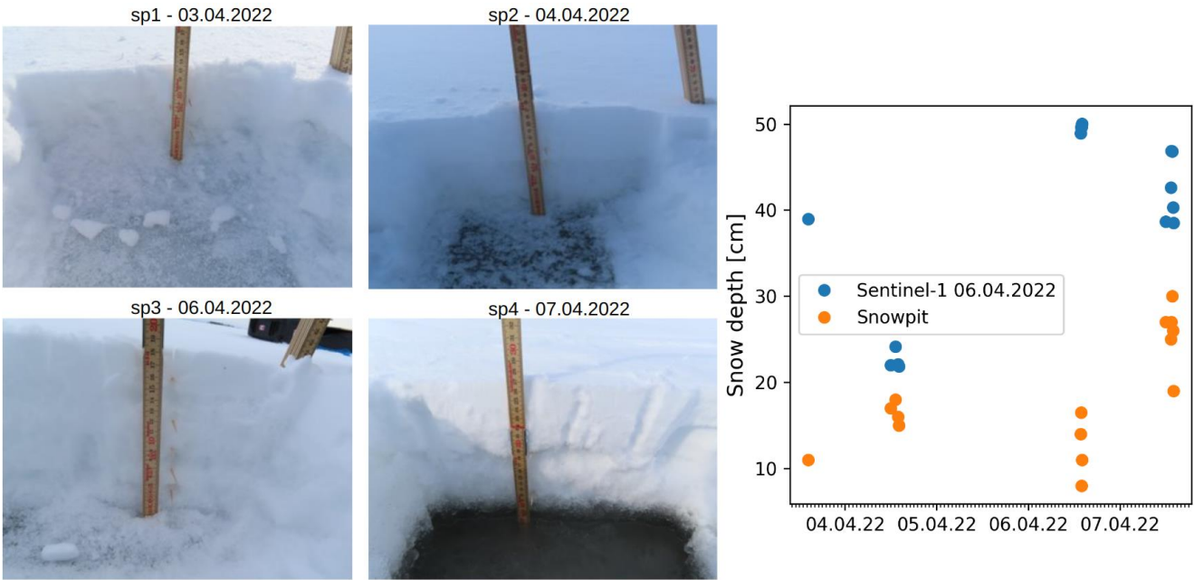
Figure S2: In situ measurements of snow depths from the snow pits (sp1 to sp4) compared to Sentinel-1 estimative at the same locations.
