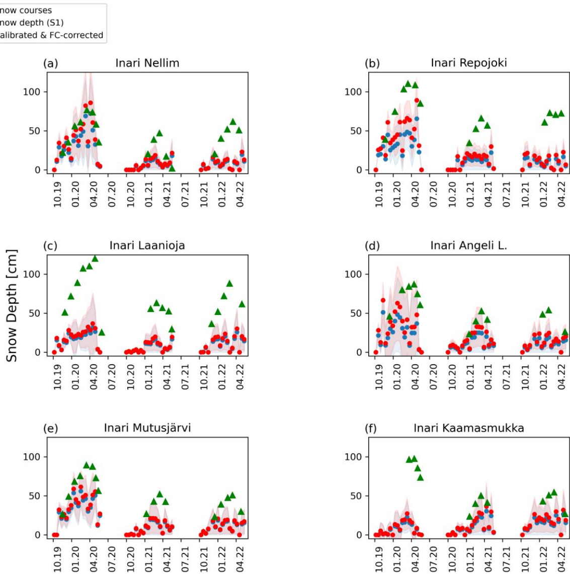
10 Figure S3: Snow depth variation between 2019 and 2022. The green triangles are the snow course measurements, the blue 11 dots represent the snow depth variation estimated from the S1 images before the correction done due the calibration and forest 12 cover (FC) attenuation. Corrected values are represented by the red dots. The uncertainty ranges are represented by the light 13 blue and red shading.
