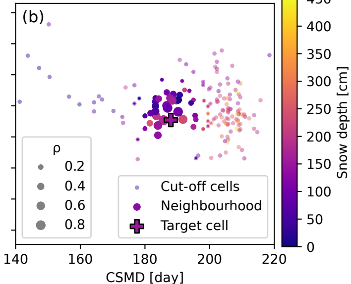
ICESat-2 feature space
