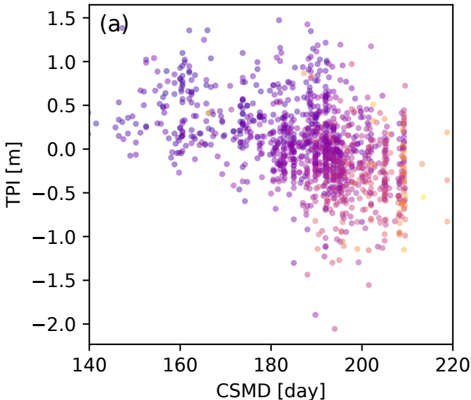
Drone maps feature space
