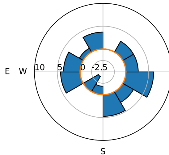
(c) P05: Jan. 15th N
