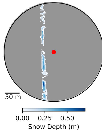
(g) P05: Jan. 15th - lidar DSM
