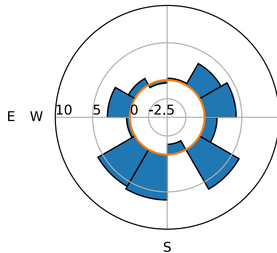
(b) P00: Jan. 15th N
