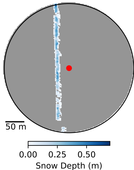
(e) P07: Jan. 15th - lidar DSM
