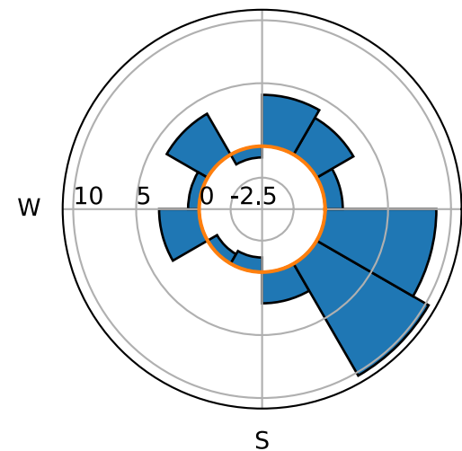
(a) P07: Jan. 15th N
