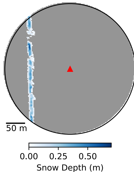
(f) P00: Jan. 15th - lidar DSM
