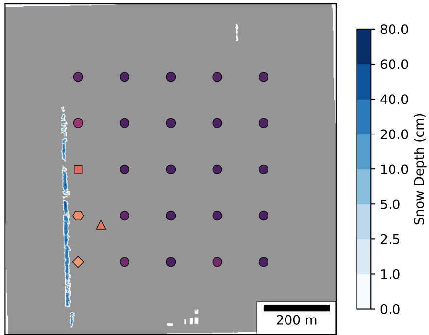
(b) Jan. 15th Snow Depths
