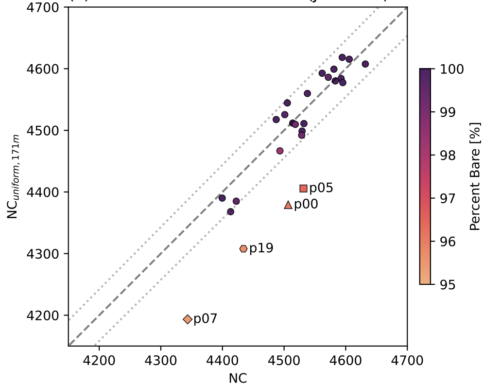
(a) Neutron Count Differences (Jan. 15th)
