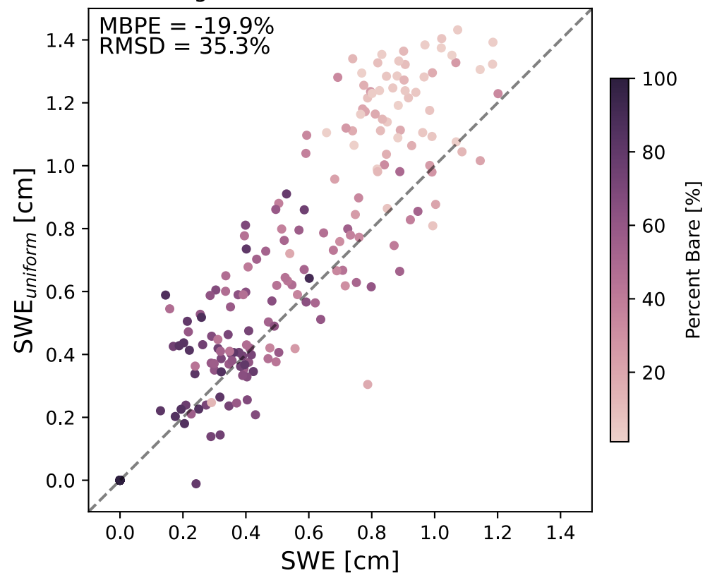
(b) SWE: Heterogeneous vs Uniform Snow
