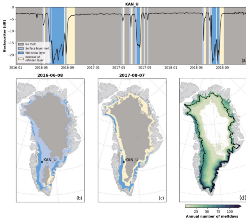
Figure 4. (a) The 2016–2018 melt detection and the backscatter signal at KAN_U. (b–c) Two examples of the spatial distribution of liquid water detection on 8 June 2016 and 7 August 2017. (d) Mean annual number of days with detected liquid water but without refreezing. In (d) we apply the maximum elevation of the snow line between 2007–2020 (black line) to mask out areas where ASCAT persistently cannot correctly detect the presence of liquid water.
