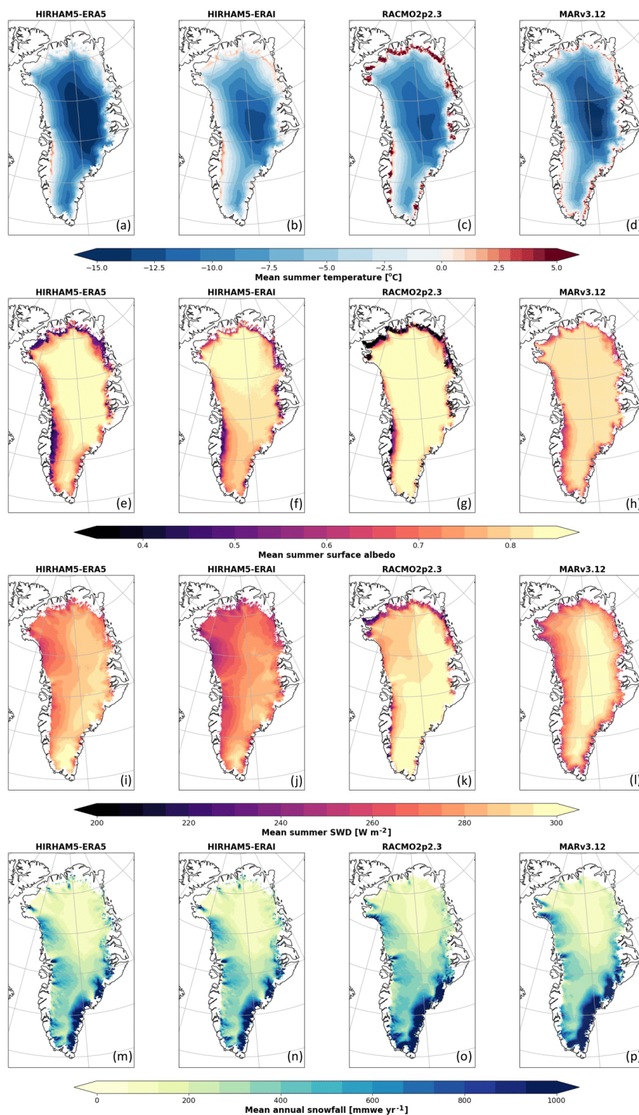
Figure 3. RCM-simulated variables from 2007–2020 for HIRHAM-ERA5, HIRHAM-ERA1, MARv3.12, and RACMO2.3p2. (a–d) Mean JJA temperatures in ^{\circ}\text{C} , (e–h) the JJA surface albedo, (i–l) the JJA downward shortwave radiation (SWD) in \text{W m}^{-2} , and (m–p) the mean annual snowfall in \text{mm w.e. yr}^{-1} .
