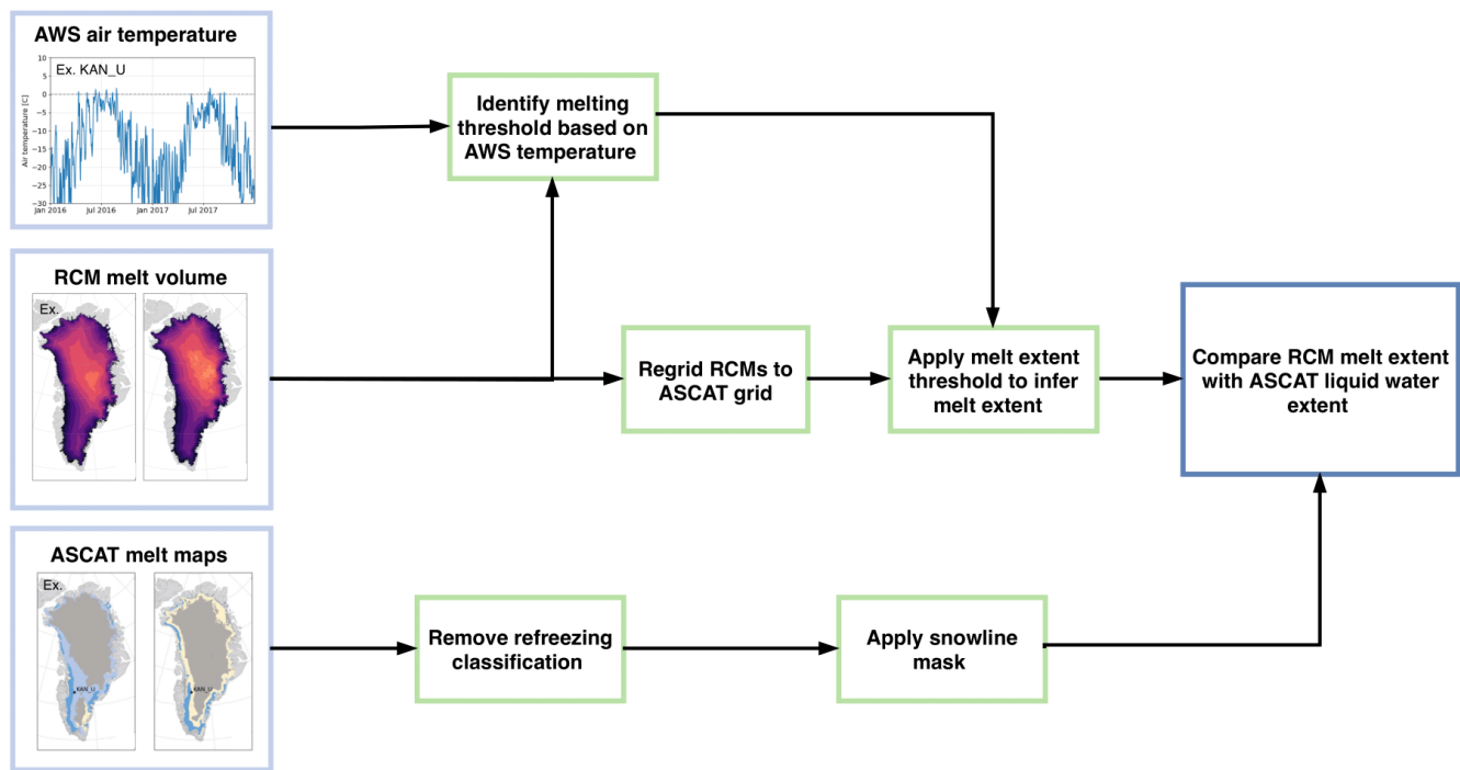
Figure 5. Diagram describing the evaluation process of RCM melt volume and processing of ASCAT wet-snow maps prior to the comparison between ASCAT liquid water extent and RCM-inferred melt extent.
