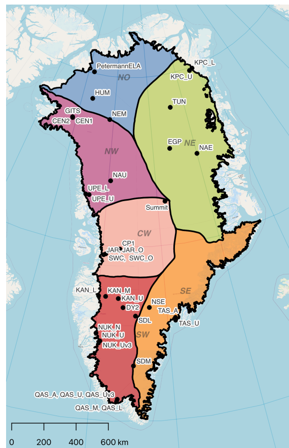
Figure 1. Locations of AWSs included in the study. Only AWSs on the ice sheet (ASCAT liquid water detection domain) are included in this study. Further, the Rignot and Mouginot (2012) drainage basins that are utilized in the subsequent evaluation of RCM-modeled melt extent against ASCAT-observed melt extent are also included.
