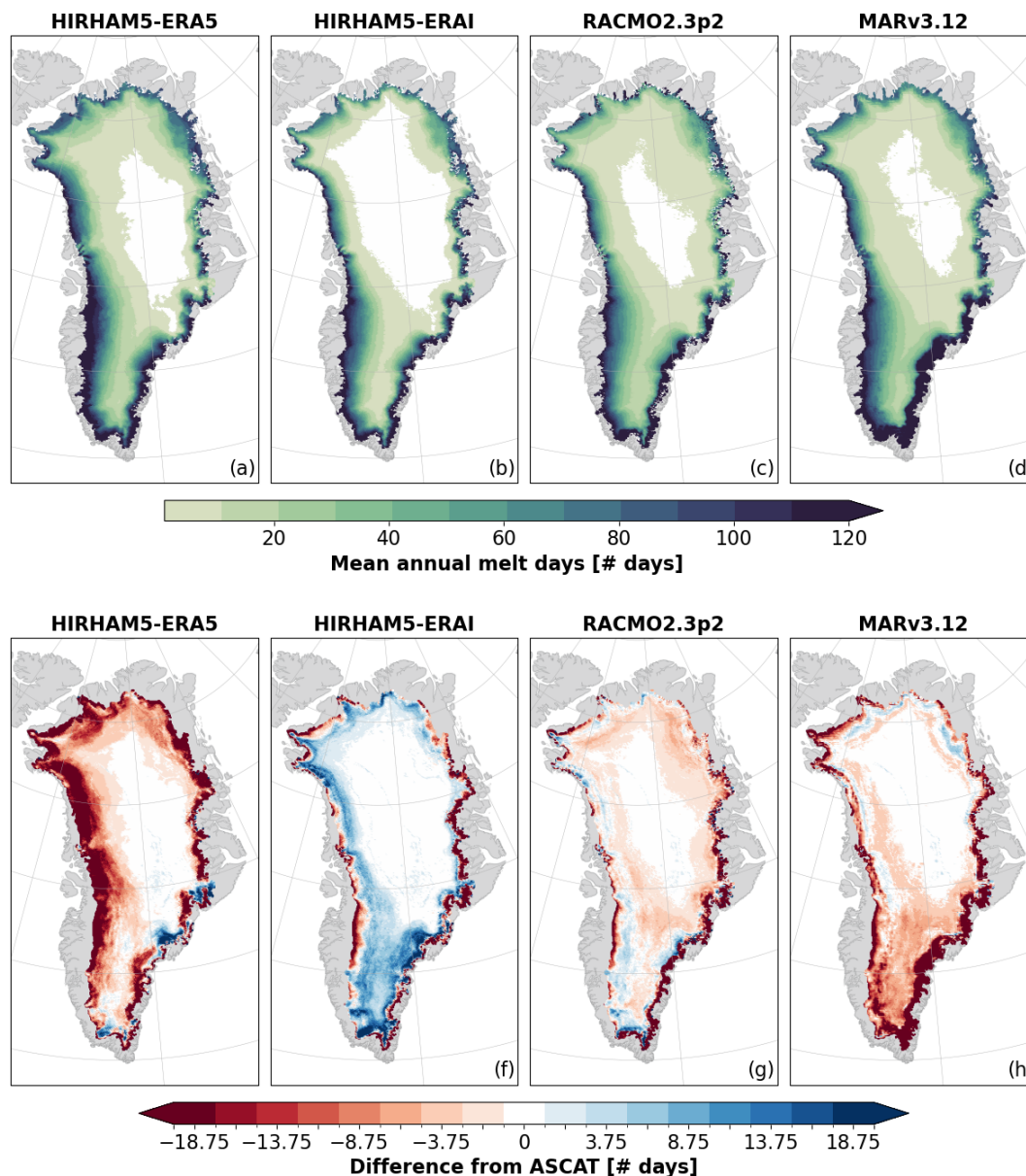
Figure A1. (a–d) The mean annual number of melt days modeled by the RCMs using a baseline threshold ( 0.1 \text{ mm w.e. d}^{-1} ) to define days with significant melt. Pixels with < 1 \text{ d} of melt on average are indicated in white, showcasing areas where melt rarely occurs. (e–h) The mean annual difference between the number of melt days in ASCAT and RCM areas above the 2007–2020 maximum snow line elevation (Fig. 4d). The red areas correspond to more melt days in ASCAT on average, and the blue areas correspond to more melt days in the RCMs on average. Melt in ASCAT is defined as ST-2A and ST-2B.
