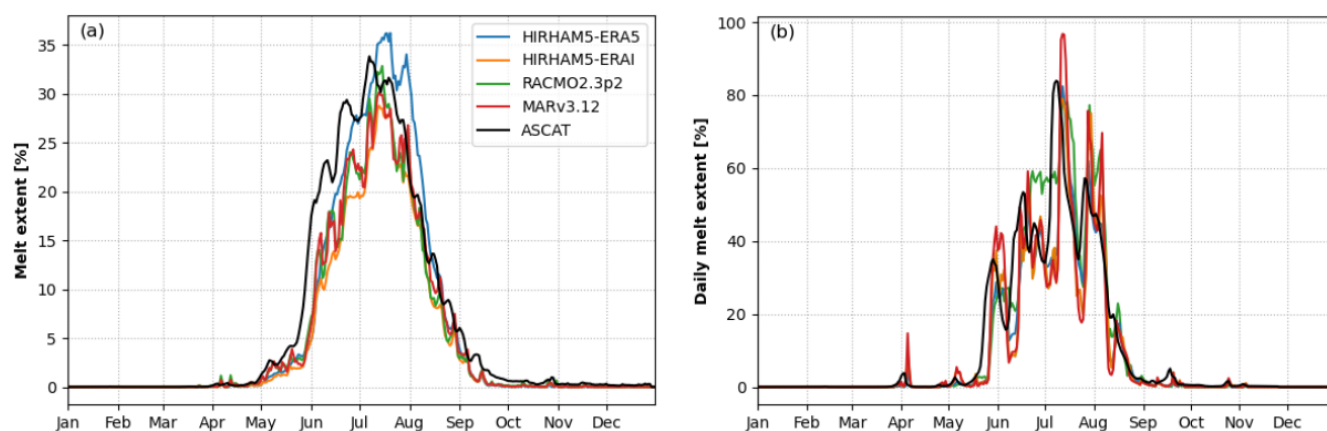
Figure 8. (a) Mean seasonal melt extent (%) modeled by RCMs using in-situ-informed thresholds and retrieved from ASCAT (2007–2020). In-situ-informed thresholds are given in Table 3. (b) Daily melt extent (%) modeled by RCMs using in-situ-informed thresholds and retrieved from ASCAT in 2012. In-situ-informed thresholds are given in Table 3. The melt extent in both (a) and (b) is constrained to areas above the maximum elevation of the snow line.
