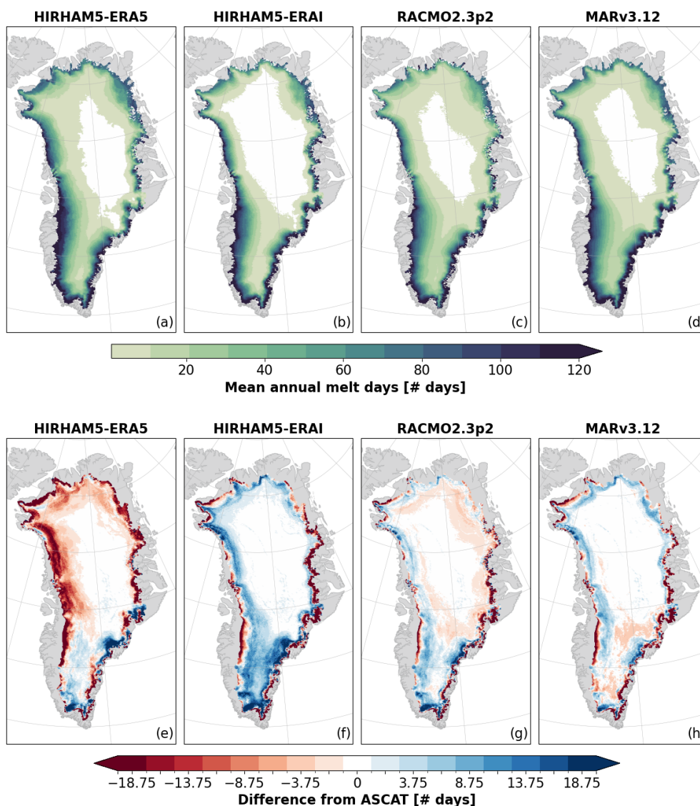
Figure 7. (a–d) The mean annual number of melt days modeled by the RCMs using an in-situ-informed melt threshold to defined days with significant melt. Pixels with < 1 d of melt on average are marked as white, showcasing areas where melt rarely occurs. (e–h) The mean annual difference between the number of melt days in ASCAT and RCMs areas above the 2007–2020 maximum snow line elevation (Fig. 4d). Red areas correspond to more melt days in ASCAT on average and blue areas correspond to more melt days in the RCM on average. Melt in ASCAT is defined as Label ST-2A and ST-2B.
