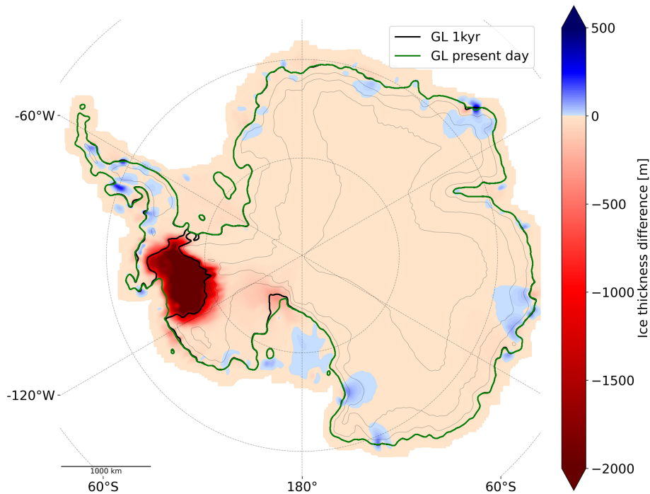
Figure 7. Future state of the Antarctic Ice Sheet using UFEMISM. Ice thickness change after a 1000-year continuation experiment initialized with present-day mass change rates. The initial modeled GL resulting from the spin-up is shown in green, and the GL position at t = 1000 years is shown in black, only where it deviates from the spin-up GL. For this figure, the UFEMISM data on an irregular triangular grid were interpolated to the same regular rectangular grid as is used in the CISM simulations and smoothed with a Gaussian kernel for visibility.
