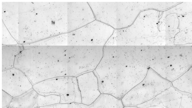
(b) 2685 m: impurity-poor ice (interglacial)
