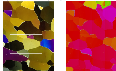
(e) 2907.5 m: impurity-rich ice
