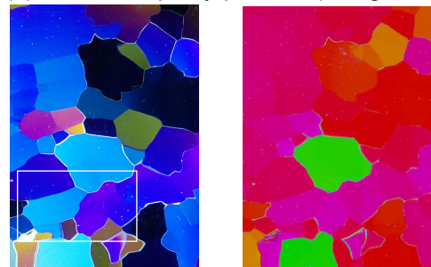
(c) 2759 m: impurity-rich ice
