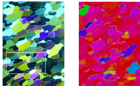
(a) 2648 m: impurity-rich ice
