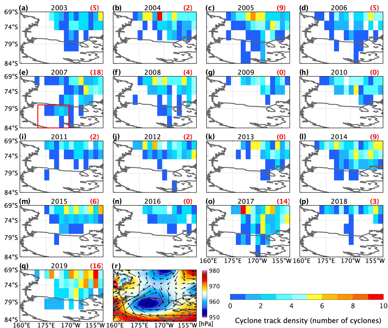
Figure 3. (a–q) Austral winter track densities (the number of tracks per section) of cyclones in the Ross Sea from 2003–2019. The red box on the Ross Ice Shelf in (e) represents the spatial extent over which the accumulated track density is calculated, and the numbers in the upper right corners indicate the density value calculated based on this box. (r) Spatial distributions of sea level pressure (colored shading) and 10 m wind vectors (black arrow) for a typical cyclone occurring on 14 August 2007.
