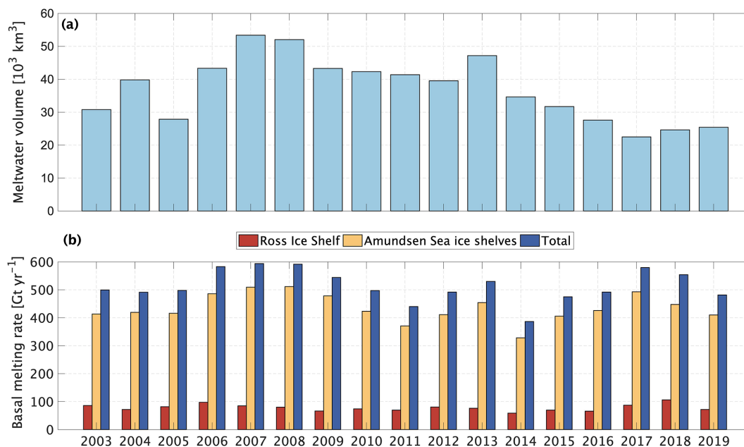
Figure 7. Time series of (a) winter-averaged ice shelf meltwater volume in the Ross Sea and (b) annual cumulative basal melting rate of the Ross Ice Shelf, the Amundsen Sea ice shelves, and their combined total from 2003 to 2019.
