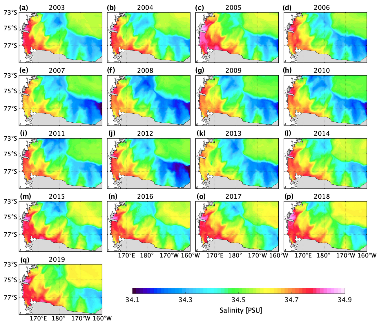
Figure 5. (a–q) Spatial distributions of depth-averaged winter salinity in the Ross Sea from 2003–2019.
