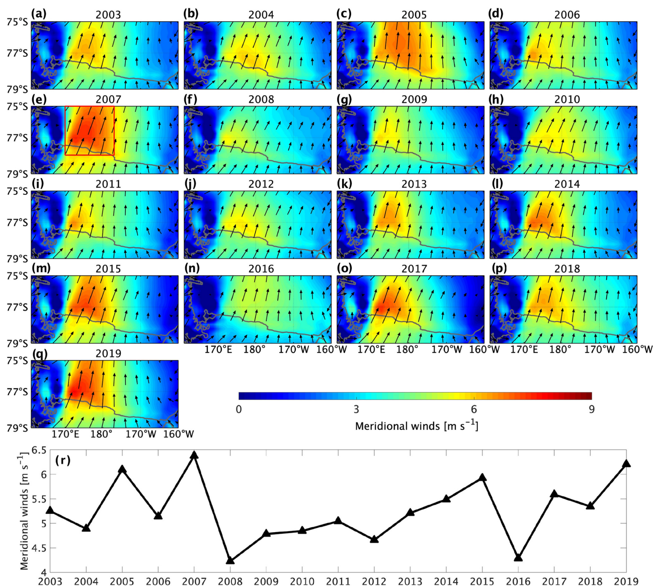
Figure 4. (a–q) Spatial distributions of winter-averaged 10 m meridional wind speed (colored shading) and 10 m wind vectors (black arrows) in the Ross Sea from 2003–2019. (r) Time series of spatially averaged meridional wind speed over the western Ross Sea (red box in panel e).
