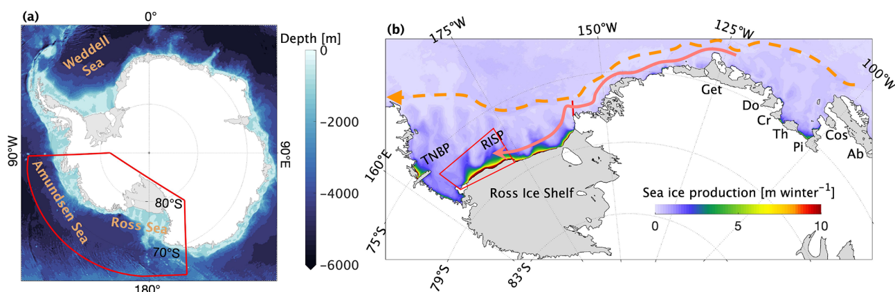
Figure 1. Geographic maps of (a) the Southern Ocean south of 60° S and (b) the Ross Sea and Amundsen Sea. Areas in white show continental surfaces, and areas in light gray indicate ice shelves. The color scale indicates accumulated sea ice production over the austral winter (June–August), averaged from 2003–2019 based on the model simulations. In panel (a), the model domain is shown by the red polygon. In panel (b), the dashed orange line indicates the Antarctic slope current, the solid pink line indicates the coastal current, and the red line between the Ross Sea and the Amundsen Sea indicates the selected transect used to calculate the freshwater transport. RISP represents the Ross Ice Shelf Polynya and TNBP indicates the Terra Nova Bay Polynya. The red box in panel (b) indicates the western RISP. The labeled local ice shelves are: Abbot Ice Shelf (Ab), Cosgrove Ice Shelf (Cos), Pine Island Ice Shelf (Pi), Thwaites Ice Shelf (Th), Crosson Ice Shelf (Cr), Dotson Ice Shelf (Do), and Getz Ice Shelf (Get).
