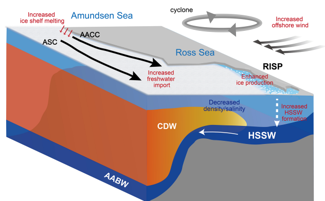
Figure 10. Schematic illustrating the atmospheric drivers of high-salinity shelf water (HSSW) production in the Ross Sea and the combined effects of HSSW production and freshwater transport from the Amundsen Sea on the Ross Sea hydrographic fields. RISP represents the Ross Ice Shelf Polynya. CDW denotes the Circumpolar Deep Water and AABW indicates the Antarctic Bottom Water. AACC represents the Antarctic coastal current and ASC refers to the Antarctic slope current.
