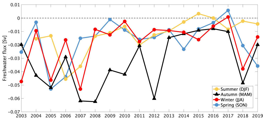
Figure 8. Time series of seasonal mean freshwater flux across the defined transect (indicated by the red line in Fig. 1b) from 2003 to 2019 for austral summer (DJF, yellow line), autumn (MAM, black line), winter (JJA, red line), and spring (SON, blue line). Negative values represent westward transport of freshwater from the Amundsen Sea into the Ross Sea.
