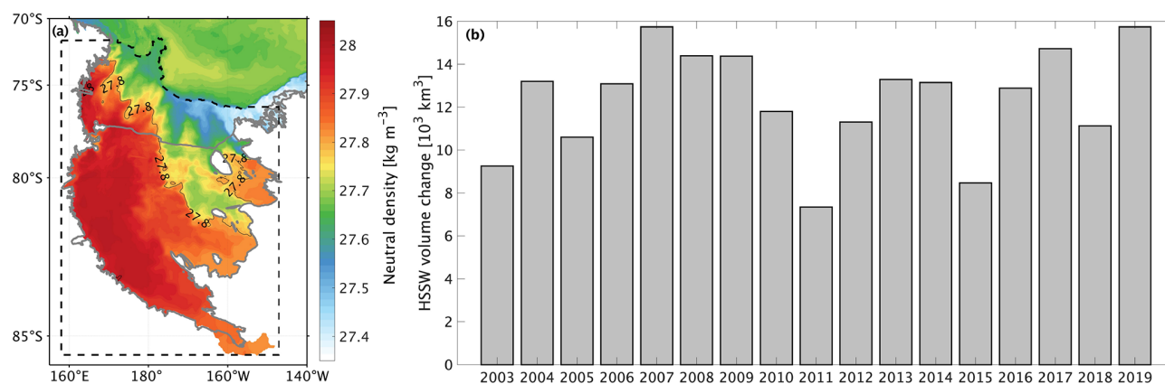
Figure 6. (a) Spatial distribution of depth-averaged neutral density (colored shading) in the Ross Sea and Ross Ice Shelf cavity. The solid gray line indicates the neutral density contour of 27.8 \text{ kg m}^{-3} . The dashed black line indicates the extent of HSSW calculated for HSSW volume; (b) Time series of HSSW volume change between July and October from 2003 to 2019.
