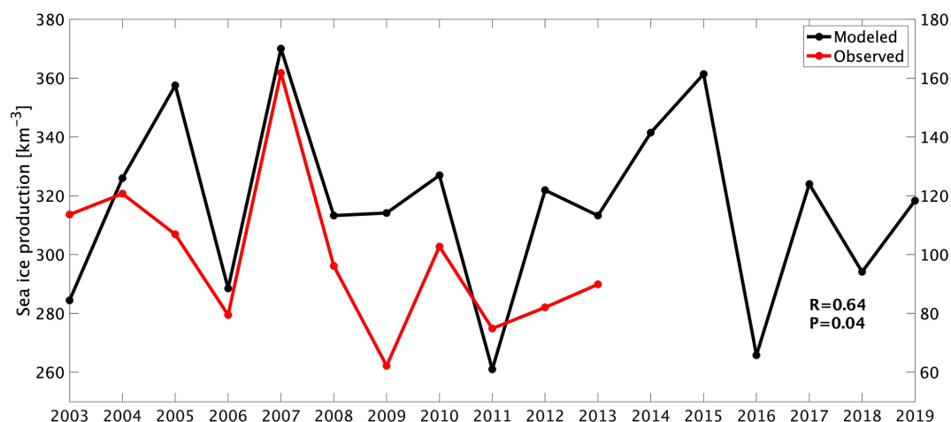
Figure 2. Time series of observed (red line; 2003–2013) and modeled (black line; 2003–2019) polynya-averaged sea ice production (SIP) during austral winter (June–August) for the western Ross Ice Shelf Polynya indicated by the red box in Fig. 1b (left y axis: modeled SIP, right y axis: observed SIP). The correlation coefficient between the observed and modeled SIP is 0.64 ( P = 0.04 ).
