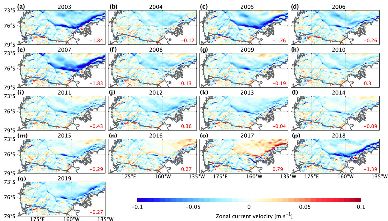
Figure 9. (a–q) Spatial distributions of winter-averaged zonal current velocities in the Ross Sea and Amundsen Sea from 2003 to 2019, averaged over the upper 300 m, where the majority of meltwater is located. The red numbers in the lower right corners indicate the volume transport of westward coastal and slope current across the defined transect (shown by the red line in Fig. 1b) and the positive values denote eastward currents.
