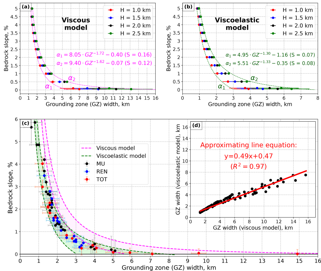
Figure 7. Modeling results of (a) viscous and (b) viscoelastic models, averaged by the thickness values, with pink and green outlines corresponding to maximum and minimum grounding zone (GZ) values for the same thickness but different inflow speeds. (c) Comparison of the modeling results (pink and green areas) with the DInSAR grounding zone measurements. (d) Correlation plot of the modeling results. Dotted green and pink lines are the same in panels (a), (b), and (c), while their equations are provided in panels (a) and (b).
