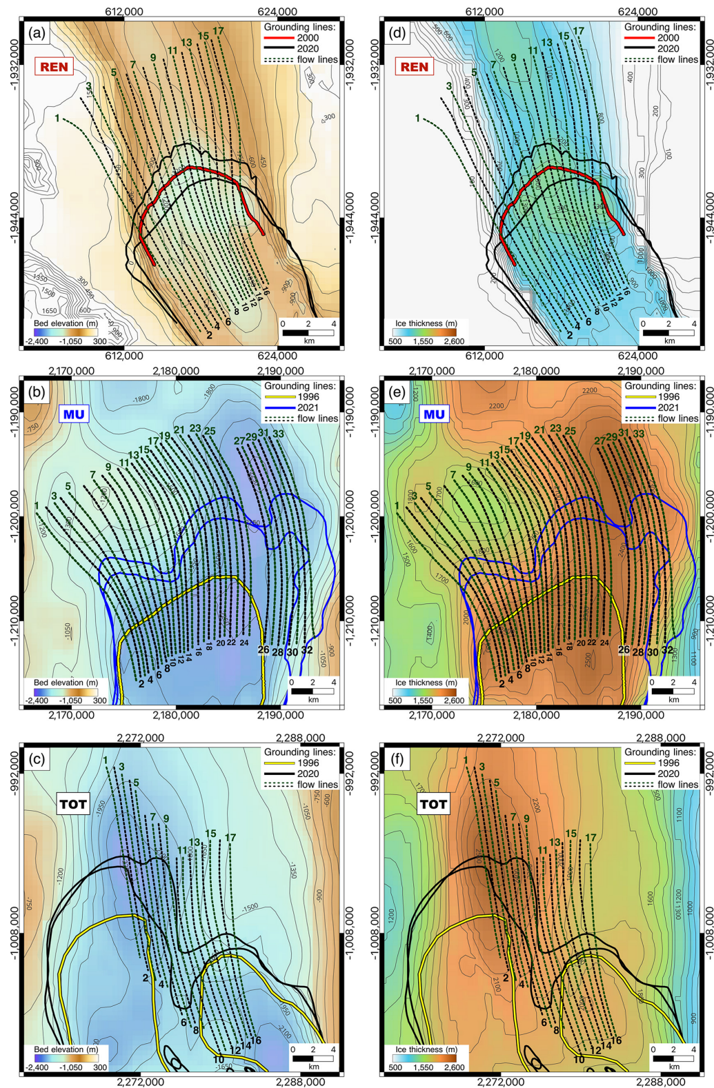
Figure 3. Bed elevation from BedMachine2 (Morlighem et al., 2017) over (a) REN, (b) MU, and (c) TOT and ice thickness maps from BedMachine2 (Morlighem et al., 2017) over (d) REN, (e) MU, and (f) TOT. The selected 69 profiles are shown as dashed green and black lines. The grounding lines over REN and TOT were mapped in 2020 (black line), while the grounding lines over MU (blue line) correspond to 2021. The grounding lines for 1996 (yellow line) and 2000 (red line) were taken from the MEaSUREs DInSAR-based Antarctic grounding line dataset (Rignot et al., 2016). All maps are represented in Antarctic projection (EPSG:3031).
