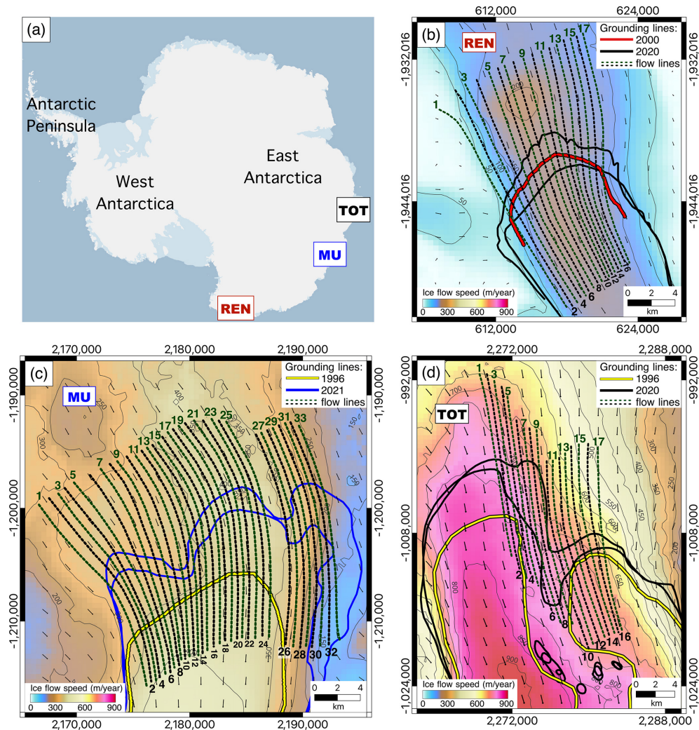
Figure 2. Study area: (a) location of TOT, MU, and REN in Antarctica and ice velocity map over (b) REN, (c) MU, and (d) TOT. The selected 69 profiles are shown as dashed green and black lines over the black ice flow vectors, derived from the MEaSUREs InSAR-based ice velocity map of Antarctica (Rignot et al., 2017). For visualization purposes, the flow vectors shown here were calculated over a velocity flow map resampled at 2 km, while the directions of the profiles were determined over the original 450 m resolution flow map to maximize the accuracy of the flow direction definition. The grounding lines over REN and TOT were mapped in 2020 (black line), while the grounding lines over MU (blue line) correspond to 2021. The grounding lines for 1996 (yellow line) and 2000 (red line) were taken from the MEaSUREs DInSAR-based Antarctic grounding line dataset (Rignot et al., 2016). All maps are represented in Antarctic projection (EPSG:3031).
