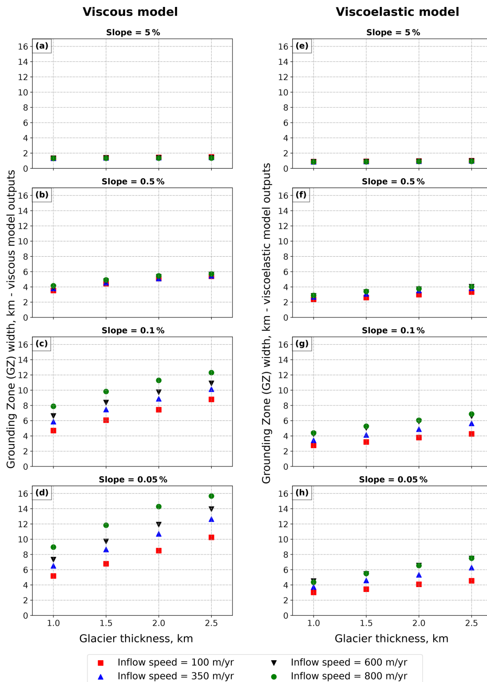
Figure 6. Dependence of the grounding zone width from the glacier thickness for inflow speeds of 100, 350, 600, and 800 \text{ m yr}^{-1} and bed slopes of 5 %, 0.5 %, 0.1 %, and 0.05 % for both viscous (a–d) and viscoelastic models (e–h). Corresponding bed slope is written above each panel, and the x axis of each panel shows the glacier thickness in kilometers, while the y axis shows the grounding zone width. Each panel contains four sets of values, colored based on the model inflow speed.
