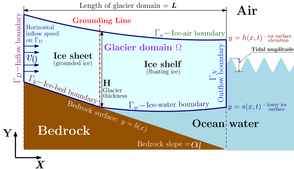
Figure 5. Model geometry for both viscous and viscoelastic problems, highlighting the ice domain \Omega boundaries, as defined in Table S3.
