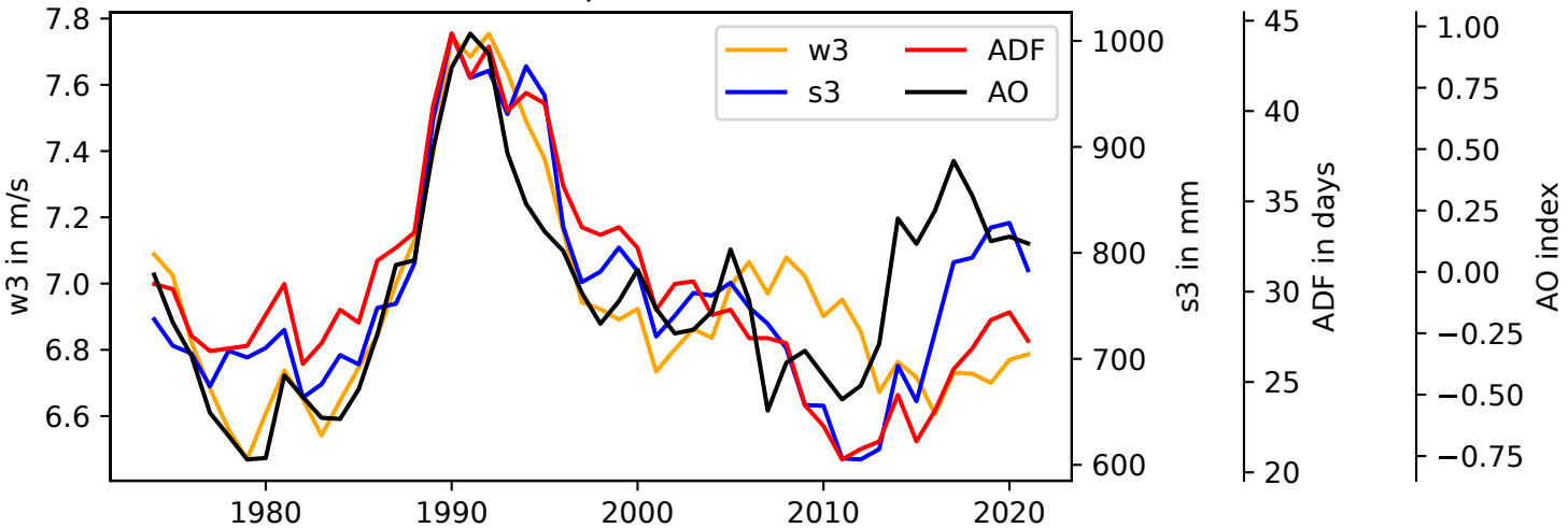
Winter ADF, AO, and predictors Nord-Troms
