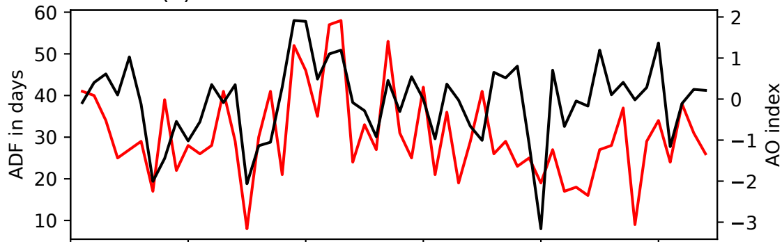
(c) 7-year rolling winter ADF and AO Nord-Troms
