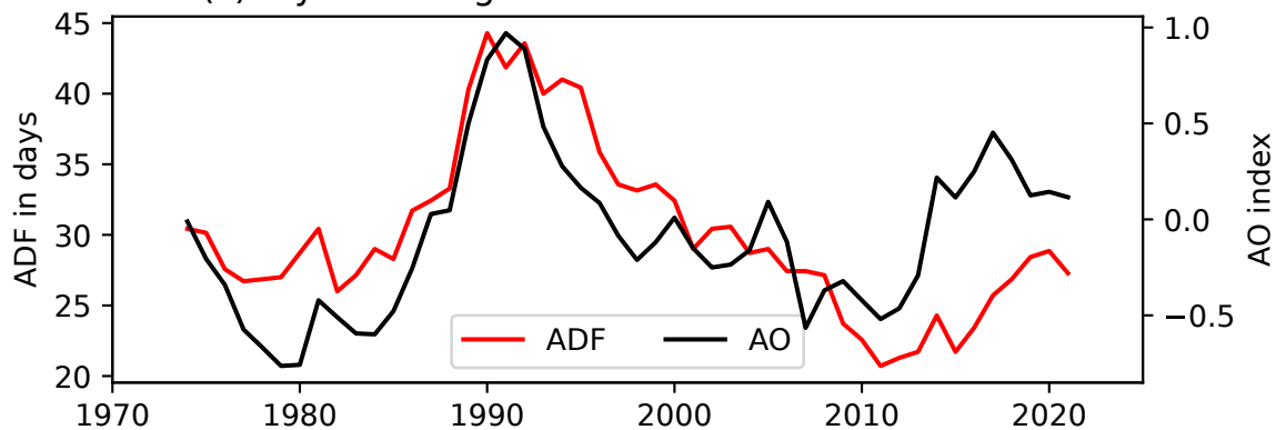
(c) 7-year rolling winter ADF and AO Nord-Troms
