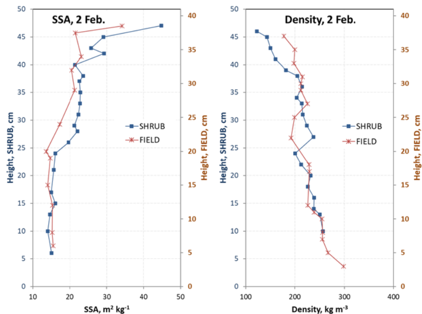
50 Figure S2. Vertical profiles of snow specific surface area and density measured at an open spot similar to FIELD and at a spot in shrubs similar to SHRUB on February 2 nd 2021.
