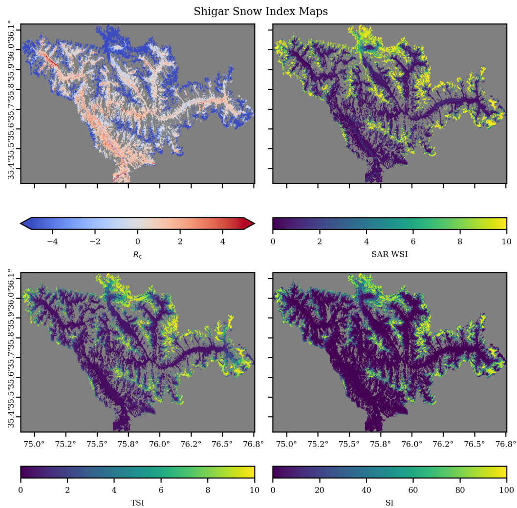
Figure S2. R_c , WSI, TSI and SI maps of Shigar.
