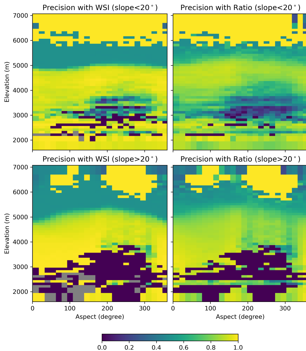
Figure S5. Precision metric aggregated by topographic bins in Hunza. Same arrangement as figure S4.
