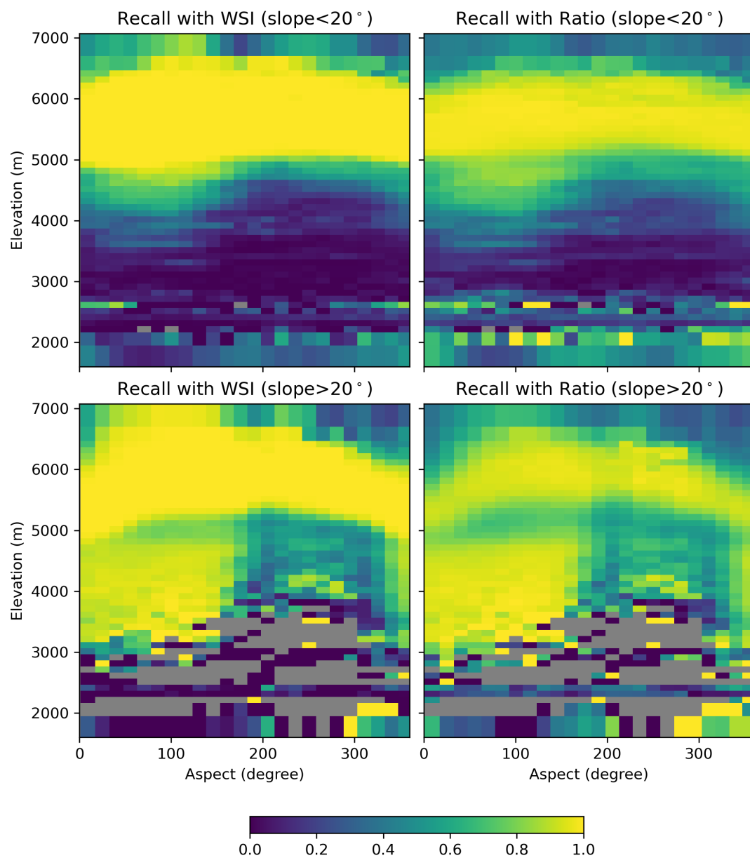
Figure S6. Recall metric aggregated by topographic bins in Hunza. Same arrangement as figure S4.
