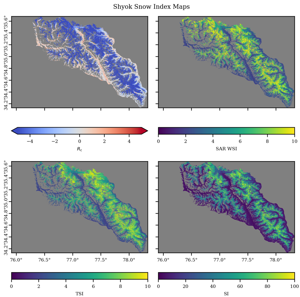
Figure S3. R_c , WSI, TSI and SI maps of Shyok.
