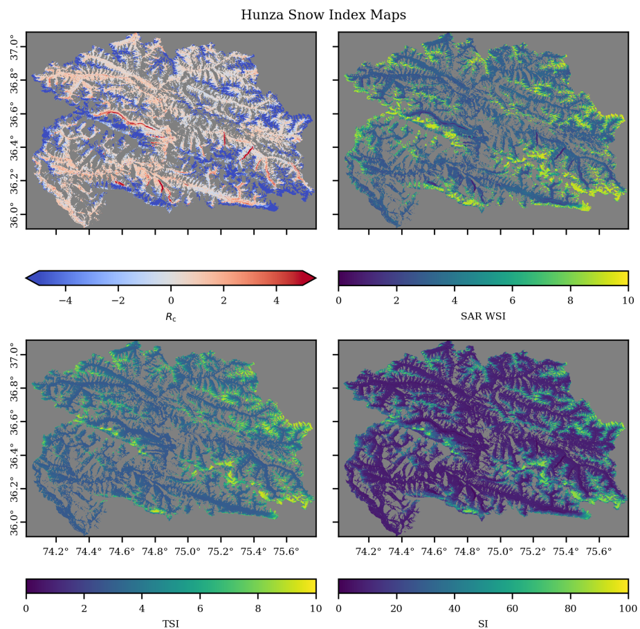
Figure S1. R_c , WSI, TSI and SI maps of Hunza.
