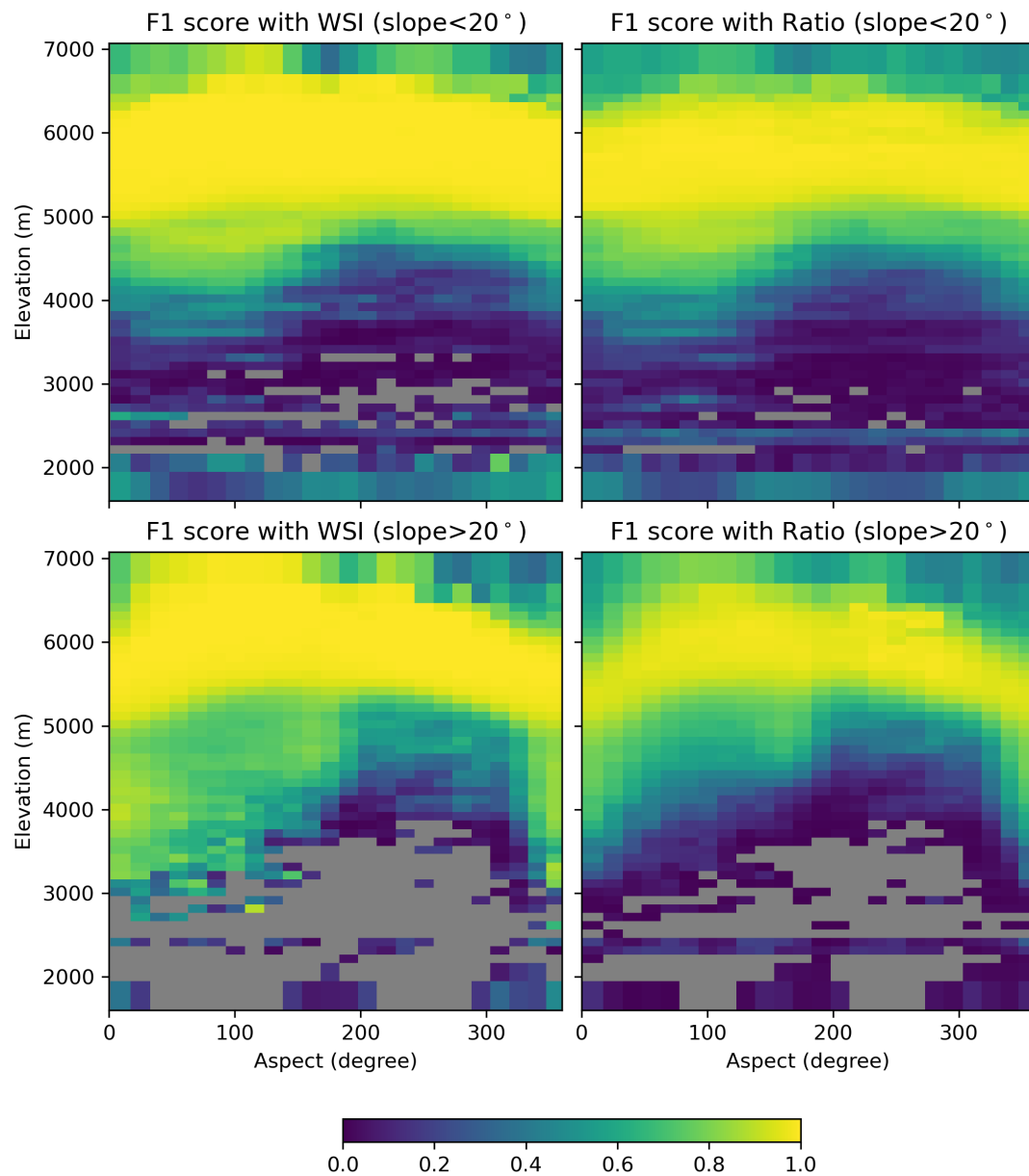
Figure S4. F1 score aggregated by topographic bins in Hunza. Top rows are with slope < 20 degrees, and bottom rows are with slope > 20 degrees. Missing values are indicated with gray.
