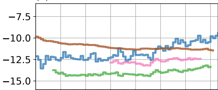
(c) Dry-snow area
