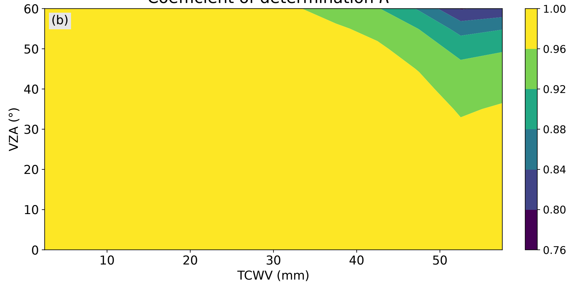
Coefficient of determination R^2
