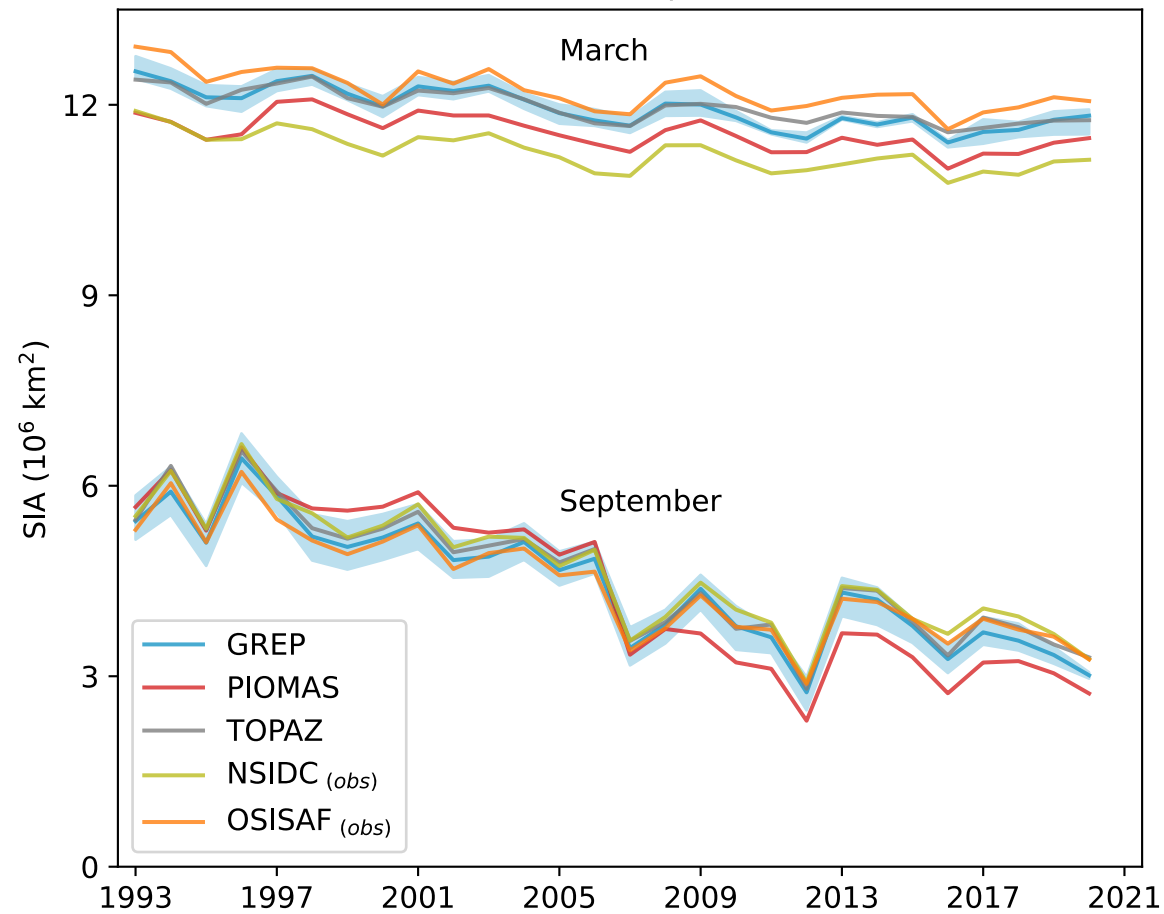
(a) March and September SIA
