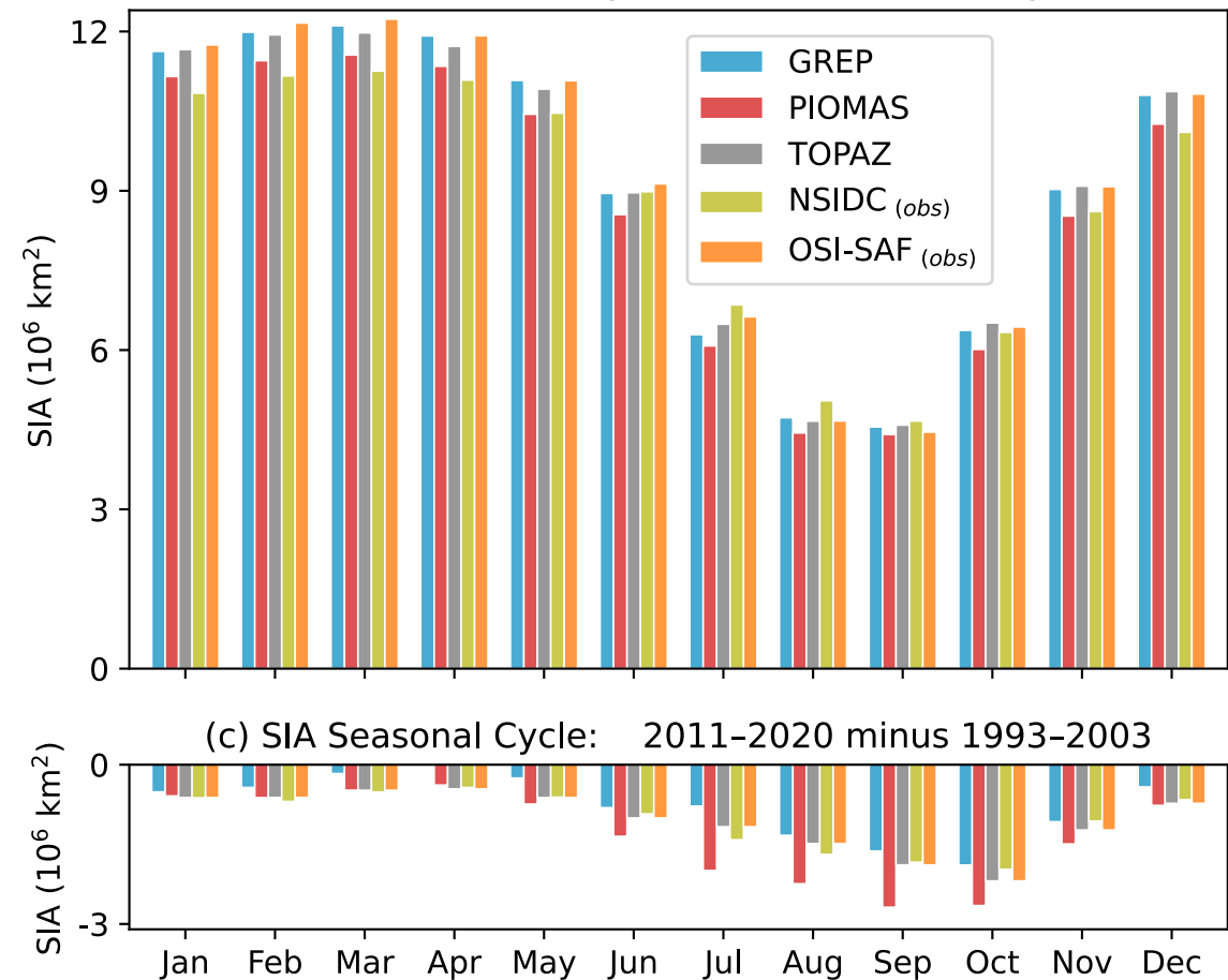
(b) SIA Seasonal Cycle: 1993-2020 Average
