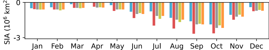
(c) SIA Seasonal Cycle: 2011-2020 minus 1993-2003
