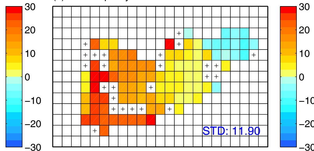
(b) Break-up Day In WRF-FLake Since 20130701
