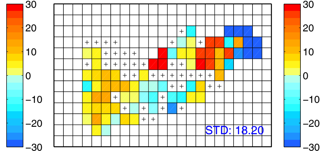
(f) Break-up Day In WRF-CLake Since 20140701
