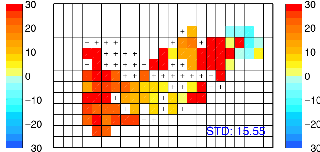
(e) Break-up Day In WRF-FLake Since 20140701
