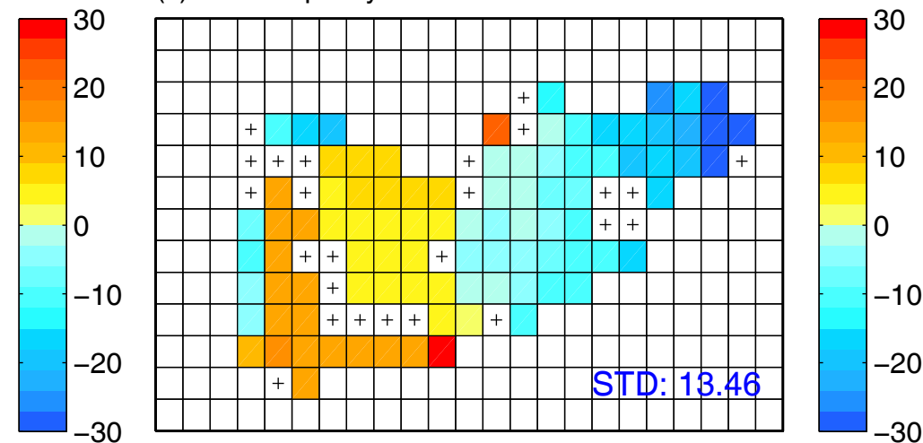
(c) Break-up Day In WRF-CLake Since 20130701
