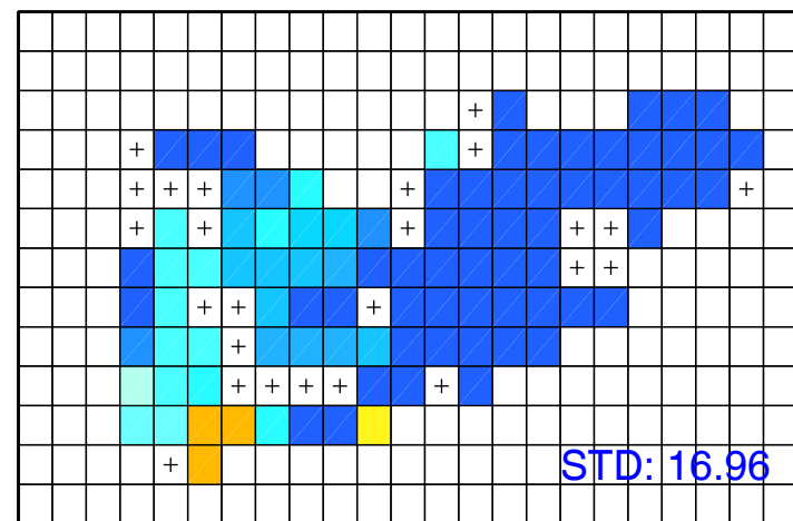
(a) Break-up Day In WRF-Ctrl Since 20130701
