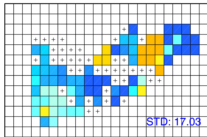
(d) Break-up Day In WRF-Ctrl Since 20140701
