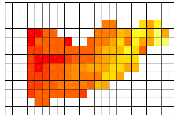
(b) Break-up Day In WRF-FLake Since 20130701
