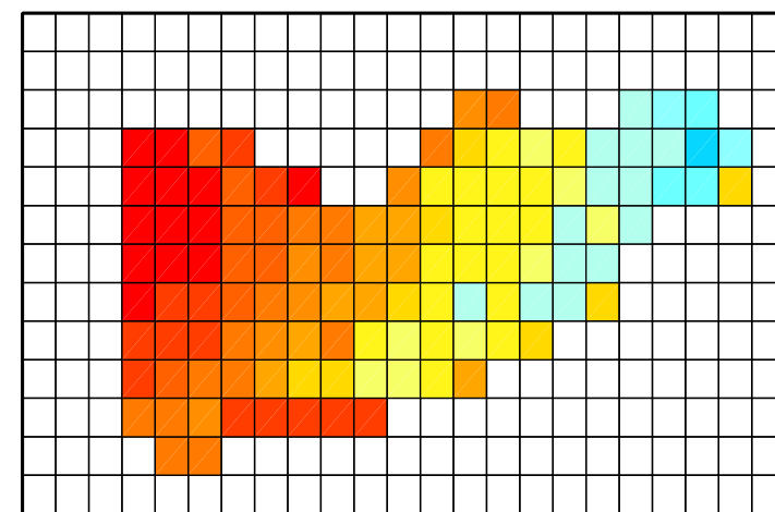
(e) Break-up Day In WRF-FLake Since 20140701
