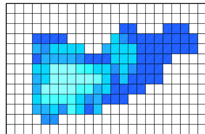
(f) Break-up Day In WRF-CLake Since 20140701
