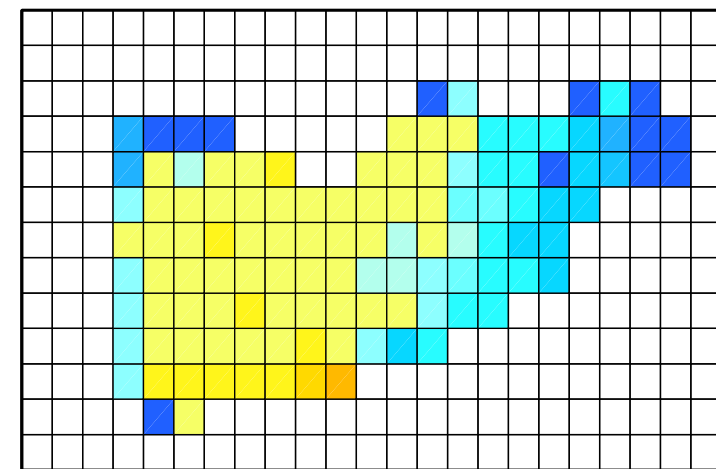
(c) Break-up Day In WRF-CLake Since 20130701
