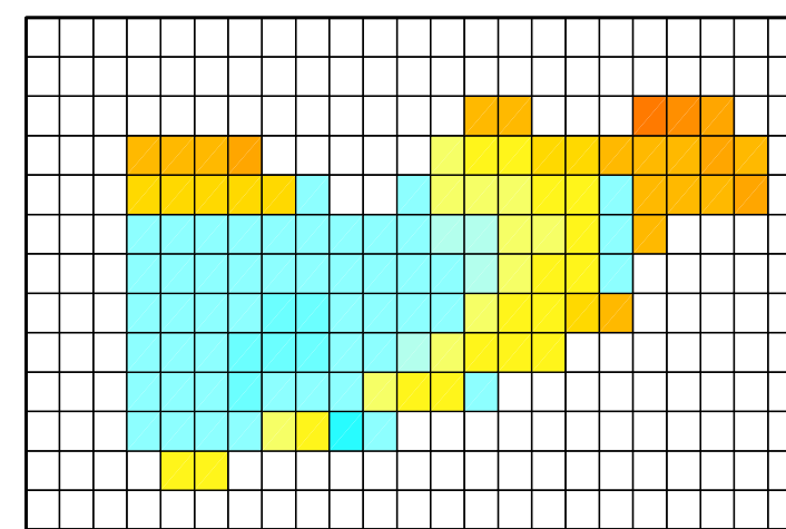
(f) Freeze-up Day In WRF-CLake Since 20140701
