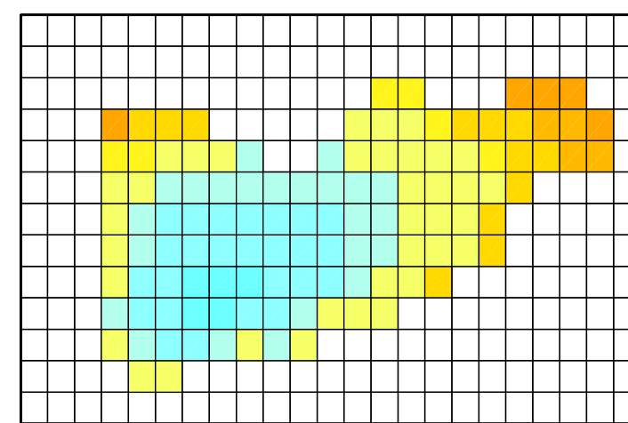
(c) Freeze-up Day In WRF-CLake Since 20130701
