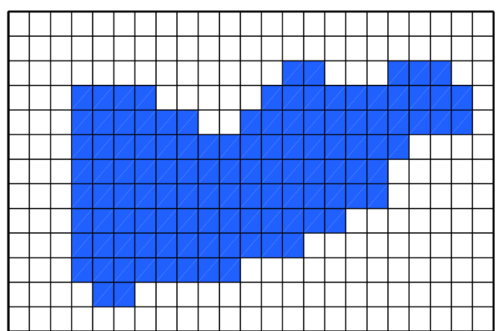
(a) Freeze-up Day In WRF-Ctrl Since 20130701
