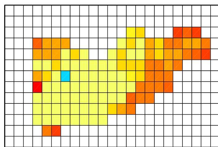
(b) Freeze-up Day In WRF-FLake Since 20130701
