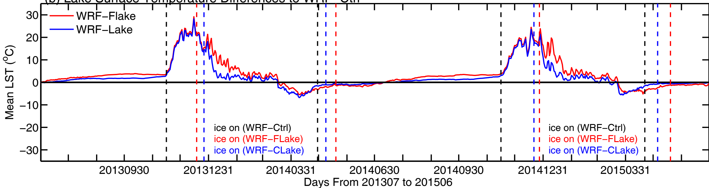
(b) Lake Surface Temperature Differences to WRF-Ctrl
