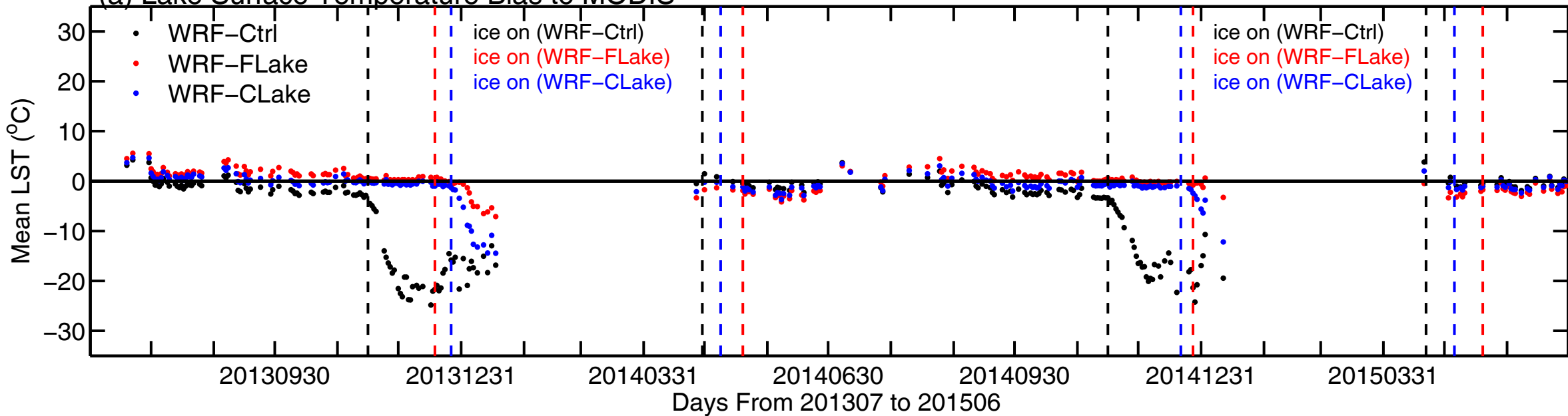
(a) Lake Surface Temperature Bias to MODIS
