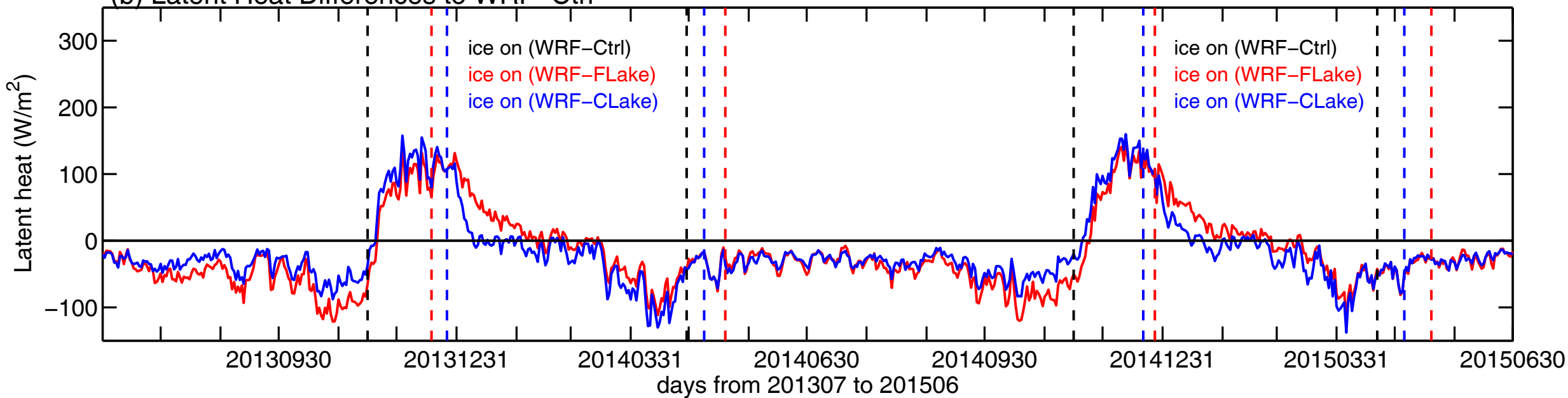
(b) Latent Heat Differences to WRF-Ctrl
