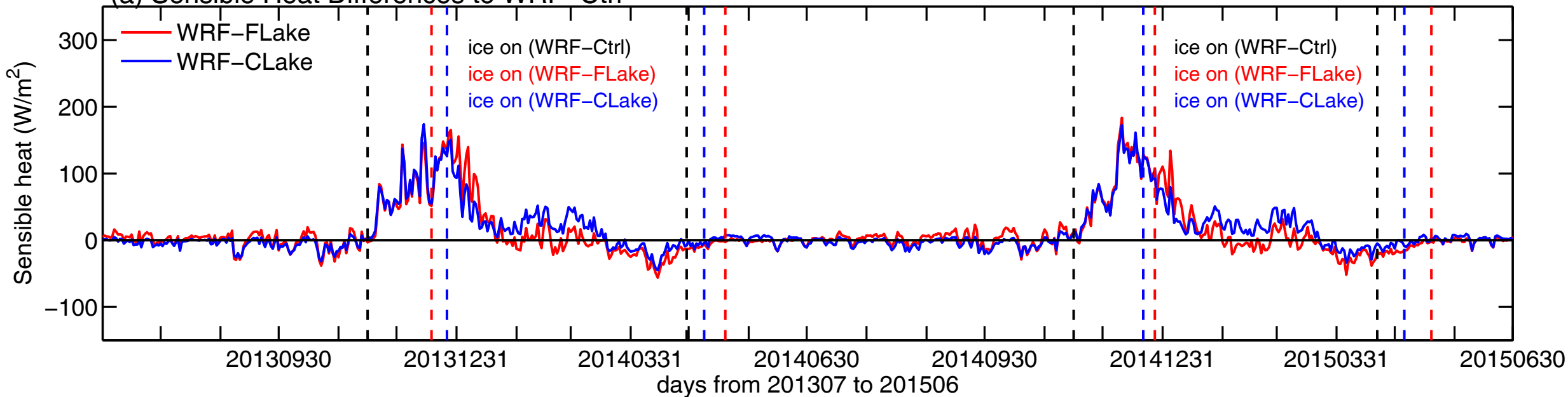
(a) Sensible Heat Differences to WRF-Ctrl
