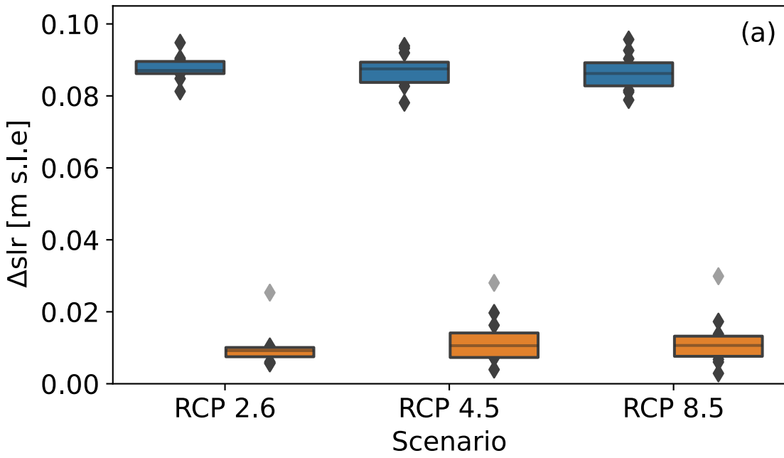
\Delta\text{slr} in 2100
