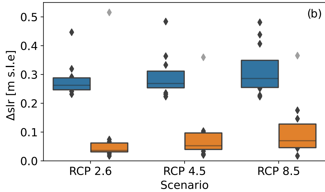
\Delta\text{slr} in 2300
