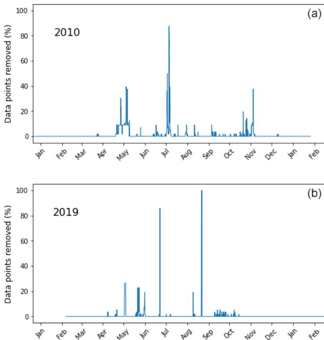
Figure 5. Data points removed using the automated data filtering routine for 2010 (a) and 2019 (b). Overall, less than 1 % of the data were removed.
