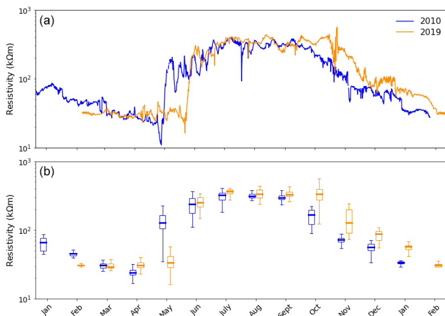
Figure 9. Average resistivity within the zone of interest ( 2 < x < 7.5 m and 0.5 < z < 1.5 m) for (a) all datasets and (b) data grouped by month. The zone of interest is plotted in Fig. 7.
