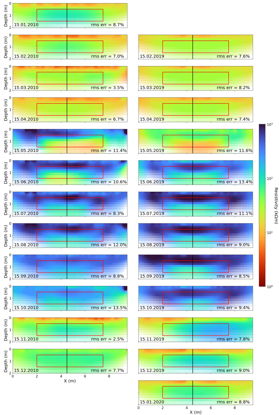
Figure 7. The 2D inverted resistivity models showing mid-month resistivity profiles for 2010 (left) and 2019 (right). The vertical black line denotes the position of the virtual borehole, and the red box denotes the zone of interest.
