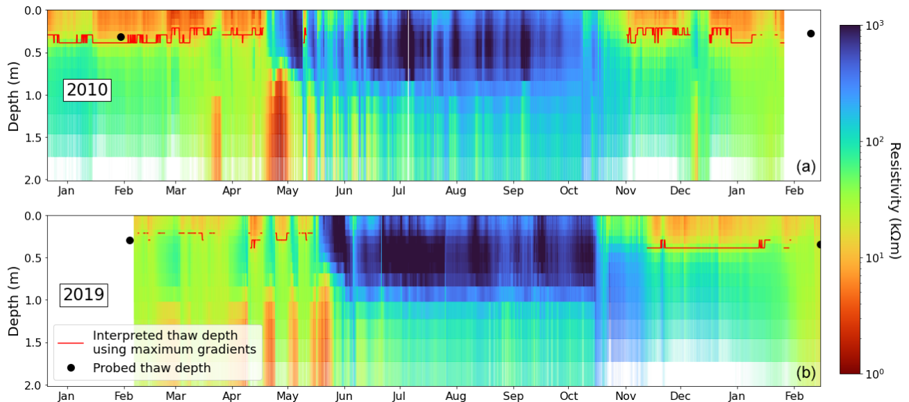
Figure 8. Inverted resistivities at a virtual borehole in the center of the ERT survey for 2010 (a) and 2019 (b) and interpreted thaw depth. Probed thaw depths are shown.
