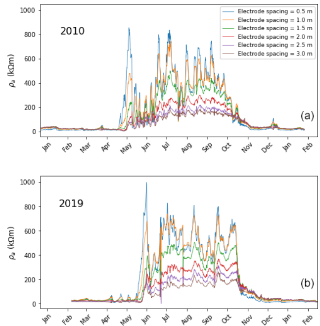
Figure 6. Apparent resistivity data of the A-ERT profile averaged for each electrode spacing for 2010 (a) and 2019 (b).
