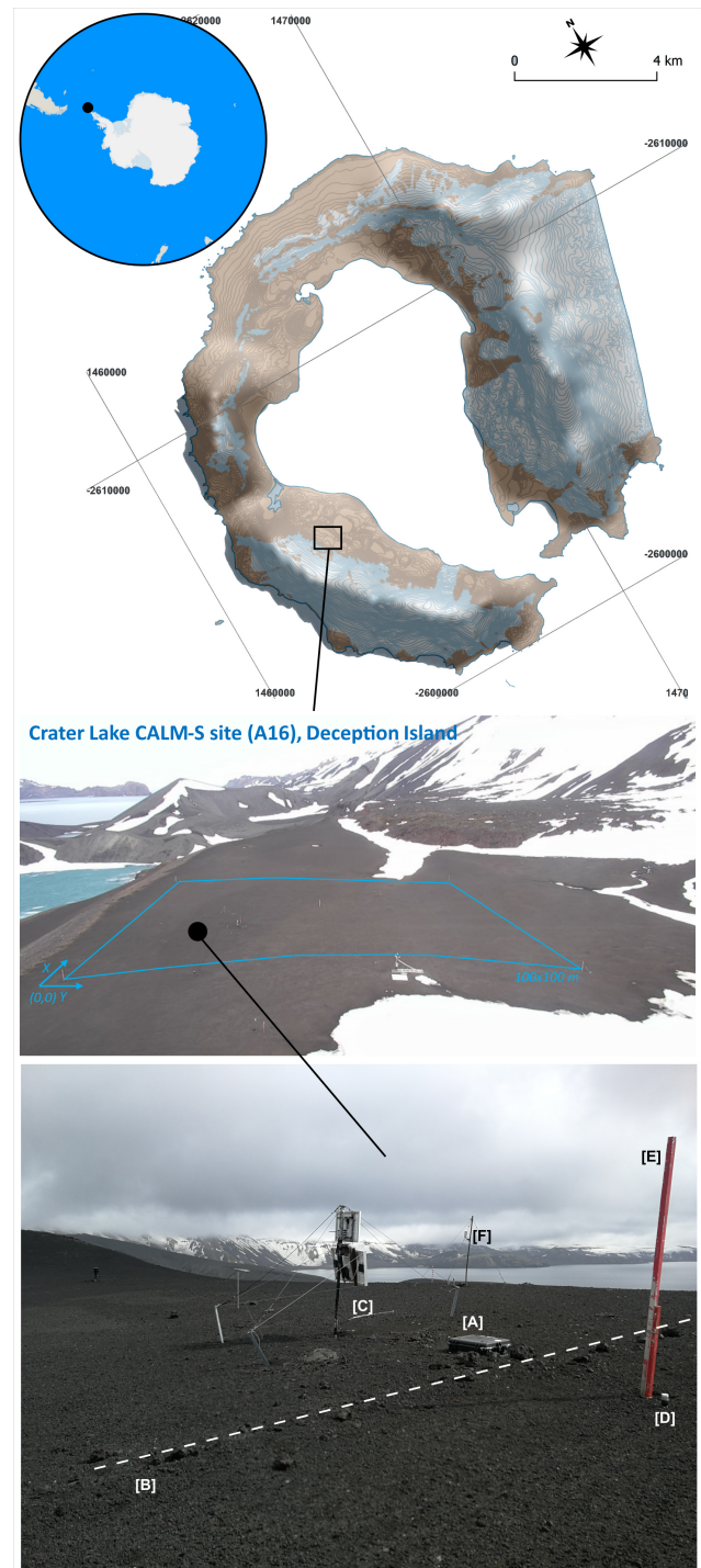
Figure 1. Location of the A-ERT setup at Crater Lake CALM-S site on Deception Island. The A-ERT box encasing the 4POINTLIGHT_10W resistivity meter instrument, solar-panel-driven battery, and multi-electrode connectors (A). Electrodes were buried in the ground and were connected to the cables (B). The solar panels are shown (C). Complementary environmental parameters are monitored close to the A-ERT profile at node x = 30 m, y = 30 m of the CALM's grid including borehole ground temperatures (D), snow thickness (E), and air temperature (F).
