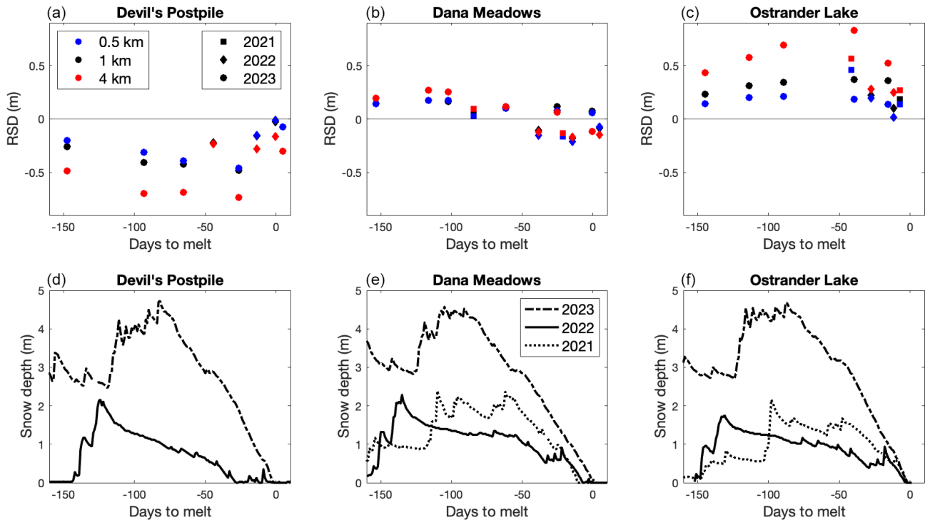
Figure 9. (a–c) Days to meltout vs. relative snow depth for all lidar surveys at select sites at all three scales. (d–f) Snow depth time series as recorded by snow stations for years with coincident lidar–station data at the selected site. Note that 2021 data are missing at Devil's Postpile.
