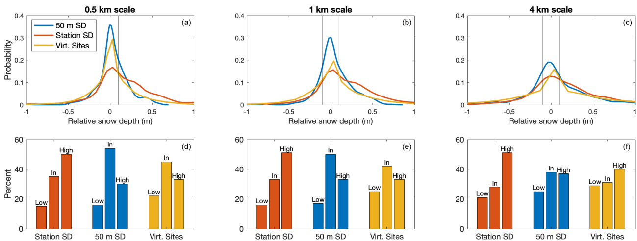
Figure 5. (a–c) Probability density functions of RSD at the 0.5, 1, and 4 km scales, using 50 m SD, station SD, and the virtual station locations as point values for all sites. (d–f) The relative distribution of RSD values that are less than -10 cm (low), within 10 cm (in), or above 10 cm (high) for each of the point values at each scale. The vertical grey lines at -0.1 and 0.1 m represent the delineations between low-biased, representative, and high-biased sites.
