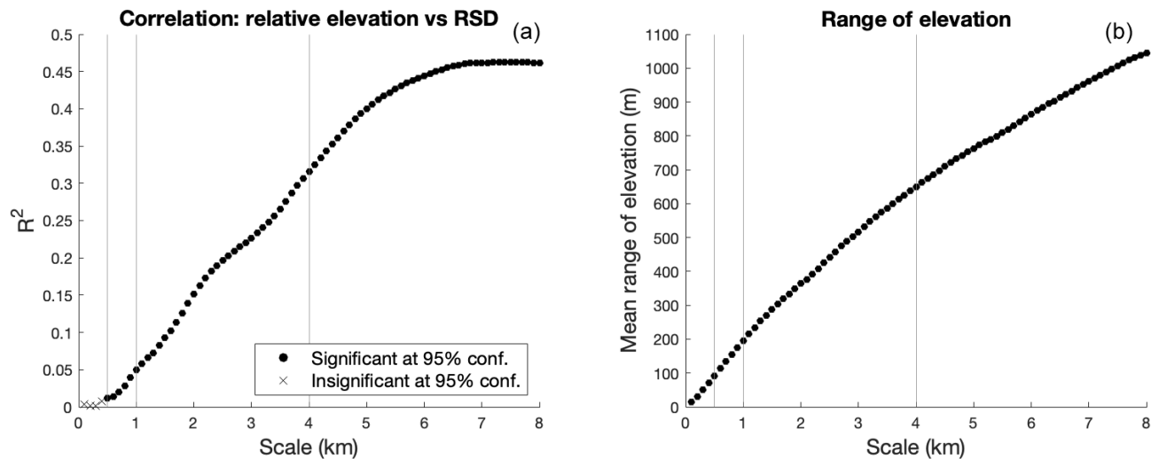
Figure 11. (a) Spatial scale vs. R^2 correlation between RSD and relative elevation. Points with p values less than 0.05 are marked with a filled circle, while sites with p values greater than 0.05 are marked with an “x” marker. (b) Scale vs. the mean range of elevations calculated from all sites.
