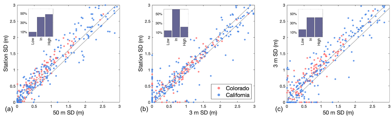
Figure 7. Scatter plots comparing the three different options for point snow depth: (a) station SD vs. 50 m SD, (b) station SD vs. 3 m SD, and (c) 3 m SD vs. 50 m SD. Points inside the black lines are within \pm 10 cm of each other. Histogram insets represent percentage of points that are below, within, or above the \pm 10 cm threshold represented by the black lines.
