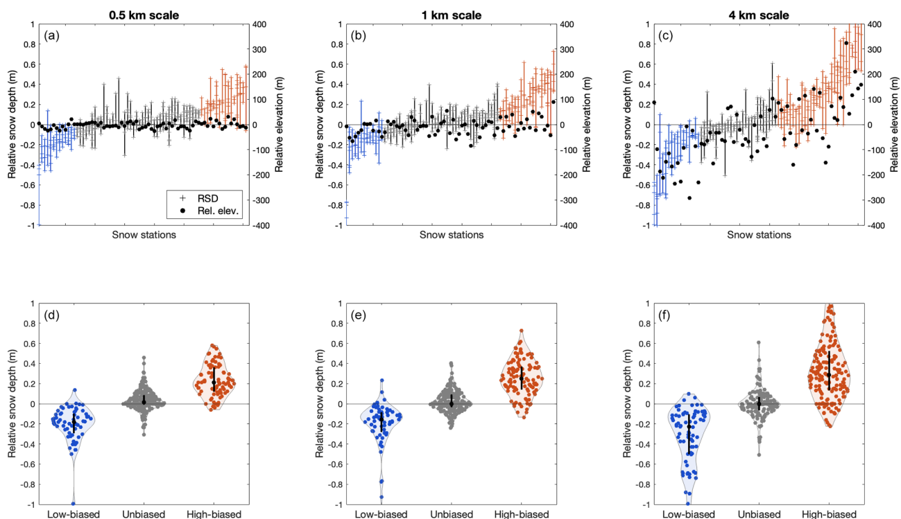
Figure 8. The temporal consistency of relative snow depth at snow stations with three or more lidar surveys. (a–c) Each snow station ( x axis) plotted against the RSD calculated from the 50 m SD for each lidar survey at 0.5, 1, and 4 km scales. Crosses represent individual RSD values, and the lines represent the range of RSD values at a given site. Stations are ordered from lowest to highest mean RSD for each scale (snow stations are thus in different orders for each scale). Relative elevation values are also plotted as black circles on the right y axis. (d–f) Distribution plots of qualitatively grouped snow stations that are typically biased low, unbiased, or biased high for the three scales. The black bars with circles represent the median and interquartile range of the RSD values.
