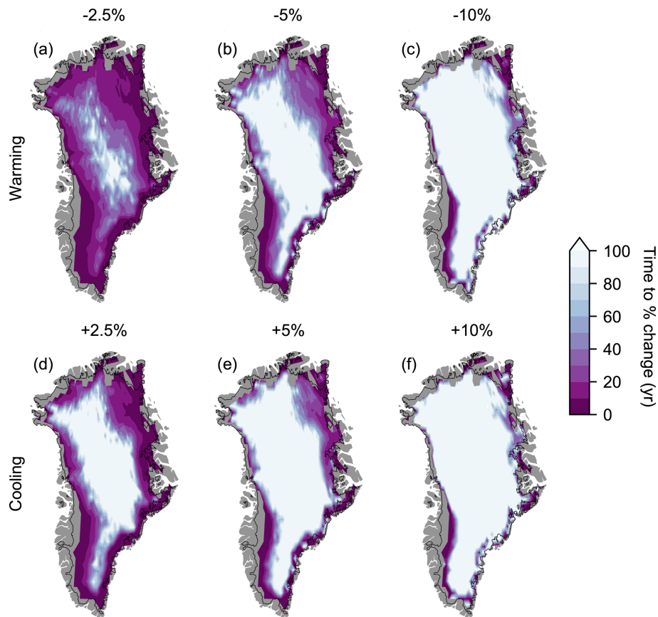
Figure 3. Elapsed time to reach a given percent change (shown above each panel) in firn air content following the control mean. Results are shown from both (a–c) warming by 1 °C and (d–f) cooling by 1 °C. The lightest shading indicates that the given percent change has not been achieved within the 100-year warming or cooling experiment, and thus the elapsed time is > 100 years. The thin black line represents the ice sheet outline. The data have been interpolated to more easily show spatial patterns. The original forcing resolution can be seen in Fig. 8.
