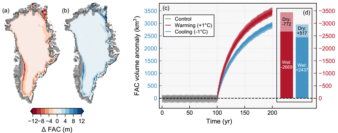
Figure 2. Change in firn air content (FAC) for the Greenland Ice Sheet calculated as the final firn air content minus the mean of the control conditions for (a) warming by 1 °C and (b) cooling by 1 °C. The thin black line represents the ice sheet outline. The data have been interpolated to more easily show spatial patterns. The original forcing resolution can be seen in Fig. 8. (c) Time series of the firn air content volume anomaly integrated over the full ice sheet for the control (gray line), warming (red line), and cooling (blue line) periods. The control period and cooling experiment use the positive values on the left y axis and the warming experiment uses the negative values on the right y axis. (d) Changes in spatially integrated firn air content in km 3 at the end of the experiments partitioned into wet firm (melt is present) and dry firm (melt is not present) areas for warming (red) and cooling (blue).
