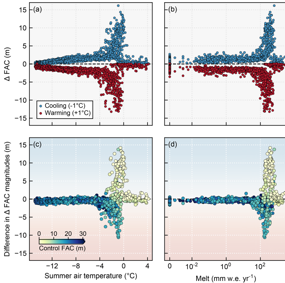
Figure 4. (a, b) The change in firn air content (FAC) for each grid cell calculated as the final value minus the control mean as a function of the control mean (a) summer air temperature and (b) melt. Blue markers indicate the effect of cooling and red indicates the effect of warming. (c, d) The difference in the magnitudes of firn air content changes due to warming and cooling. The difference is calculated as the magnitude of the cooling change minus the magnitude of the warming change such that positive values indicate a greater response to cooling (blue background shading) and negative values indicate a greater response to warming (red background shading). The markers are colored by the control mean firn air content. Note the semi-logarithmic x scales used for melt in (b) and (d).
