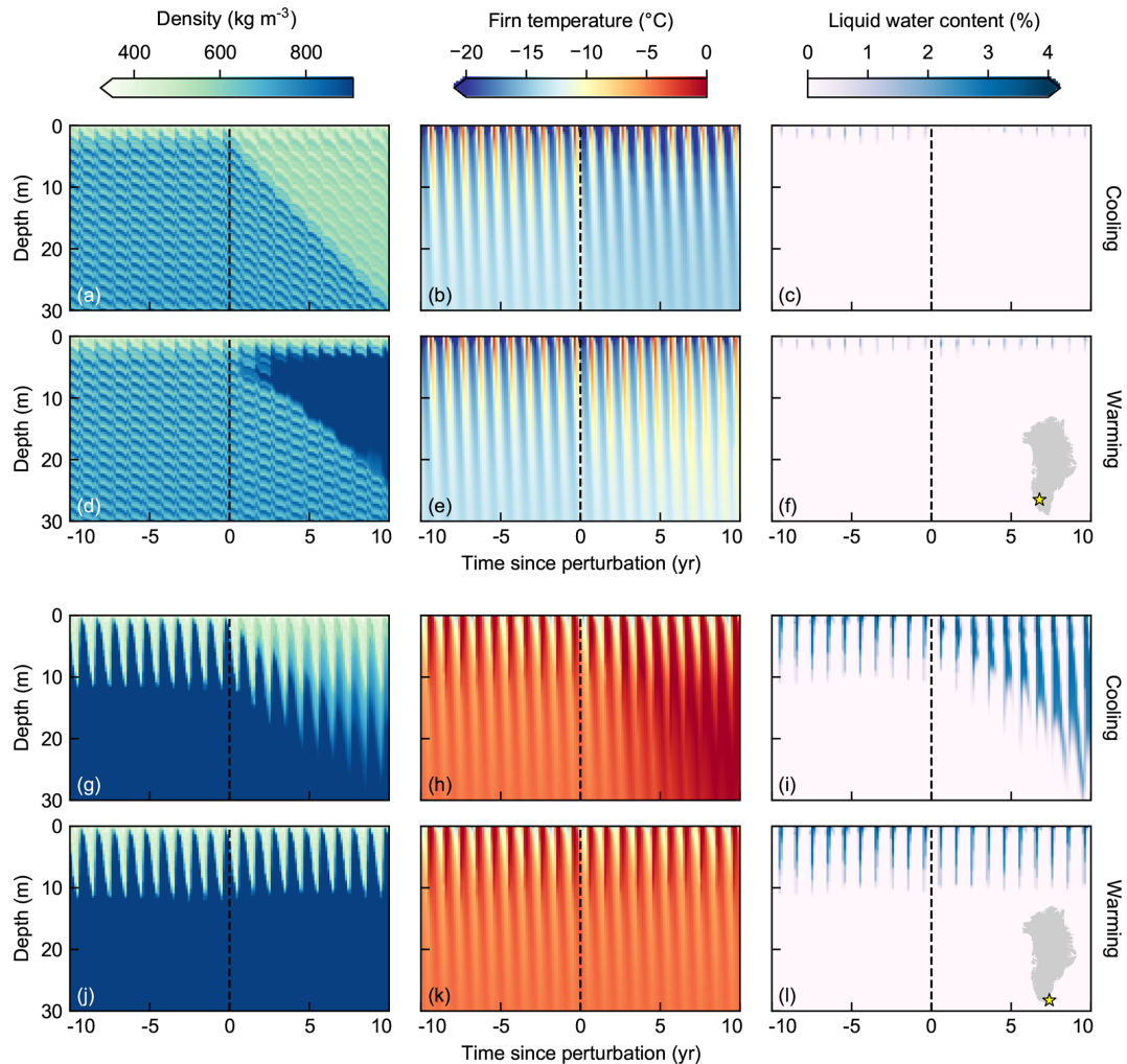
Figure 7. Time–depth plots showing firn properties (density, firn temperature, and liquid water content) for the upper 30 m of the firn column for the 10 years before and after the temperature perturbation (vertical dashed black line) for two example locations. (a–f) Results from a grid cell in southwest Greenland as seen in Fig. 6e. (g–l) Results from a grid cell in southeast Greenland as seen in Fig. 6f. The responses to cooling are shown in panels (a)–(c) and (g)–(i), and the responses to warming are shown in panels (d)–(f) and (j)–(l). Inset maps in panels (f) and (l) show each example's location on the ice sheet as a yellow star.
