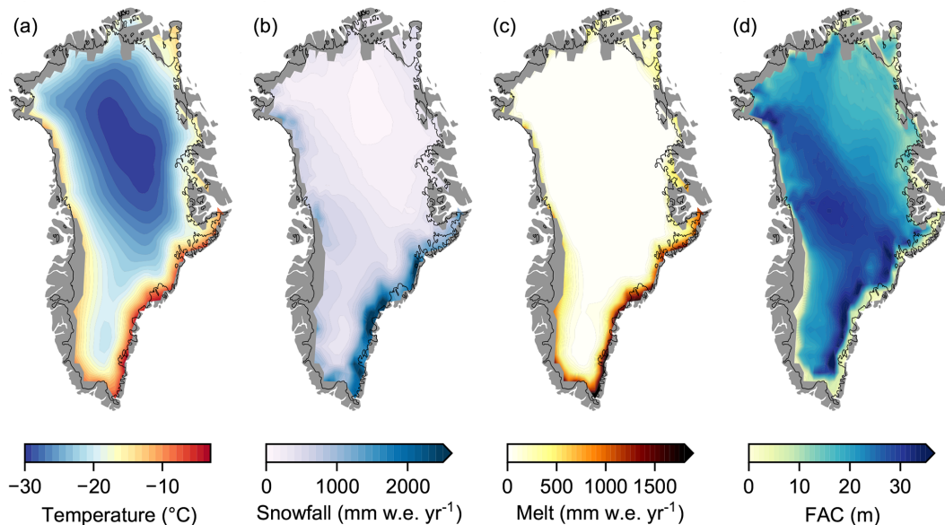
Figure 1. Greenland Ice Sheet mean annual (a) temperature, (b) snowfall, (c) melt, and (d) firn air content (FAC) from the 100-year control climate (i.e., the 1991 climate) prior to the warming and cooling experiments. The thin black line represents the ice sheet outline. The data have been interpolated to more easily show spatial patterns. The original forcing resolution can be seen in Fig. 8.
