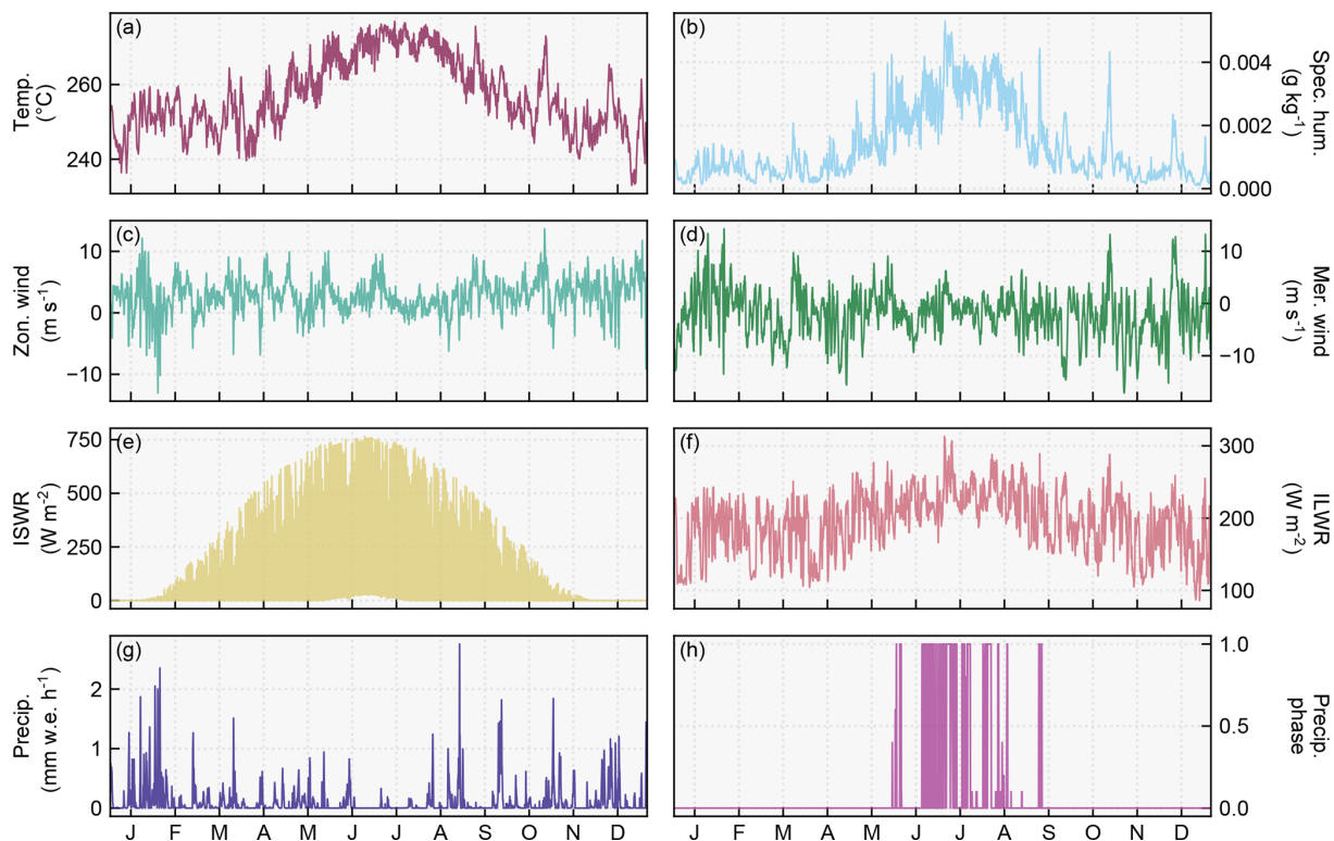
Figure A1. Example of 1 year (1991) of hourly unperturbed atmospheric forcing data for a single location ( 69.5^{\circ} N, 27.5^{\circ} W). (a) Air temperature, (b) specific humidity, (c) zonal wind, (d) meridional wind, (e) incoming shortwave radiation, (f) incoming longwave radiation, (g) precipitation, and (h) precipitation phase. The precipitation phase is a fractional value ranging from 0 to 1, where 0 is all solid precipitation and 1 is all liquid precipitation.
