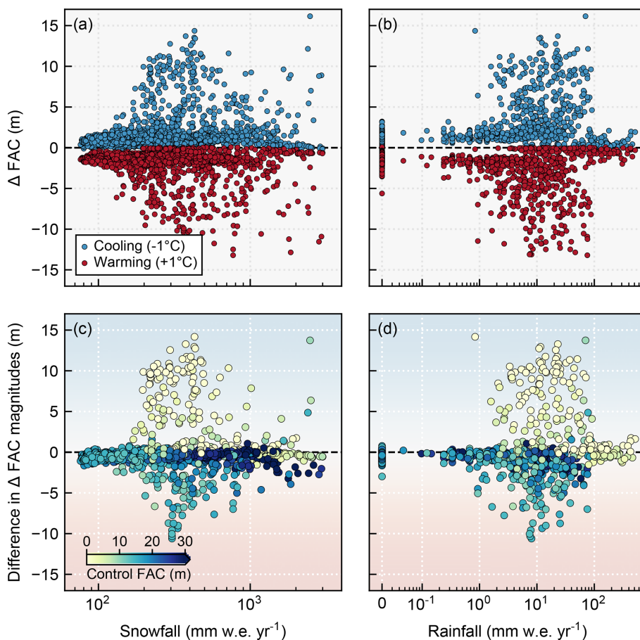
Figure A2. (a, b) The change in firn air content (FAC) for each grid cell calculated as the final value minus the control mean as a function of the control mean (a) snowfall and (b) rainfall. Blue markers indicate the effect of cooling and red indicates the effect of warming. (c, d) The difference in the magnitudes of firn air content changes due to warming and cooling. The difference is calculated as the magnitude of the cooling change minus the magnitude of the warming change such that positive values indicate a greater response to cooling (blue background shading) and negative values indicate a greater response to warming (red background shading). The markers are colored by the control mean firn air content. Note the semi-logarithmic x scales used in all panels.
