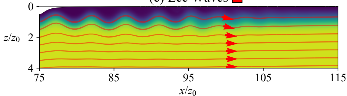
(c) Lee Waves ■
