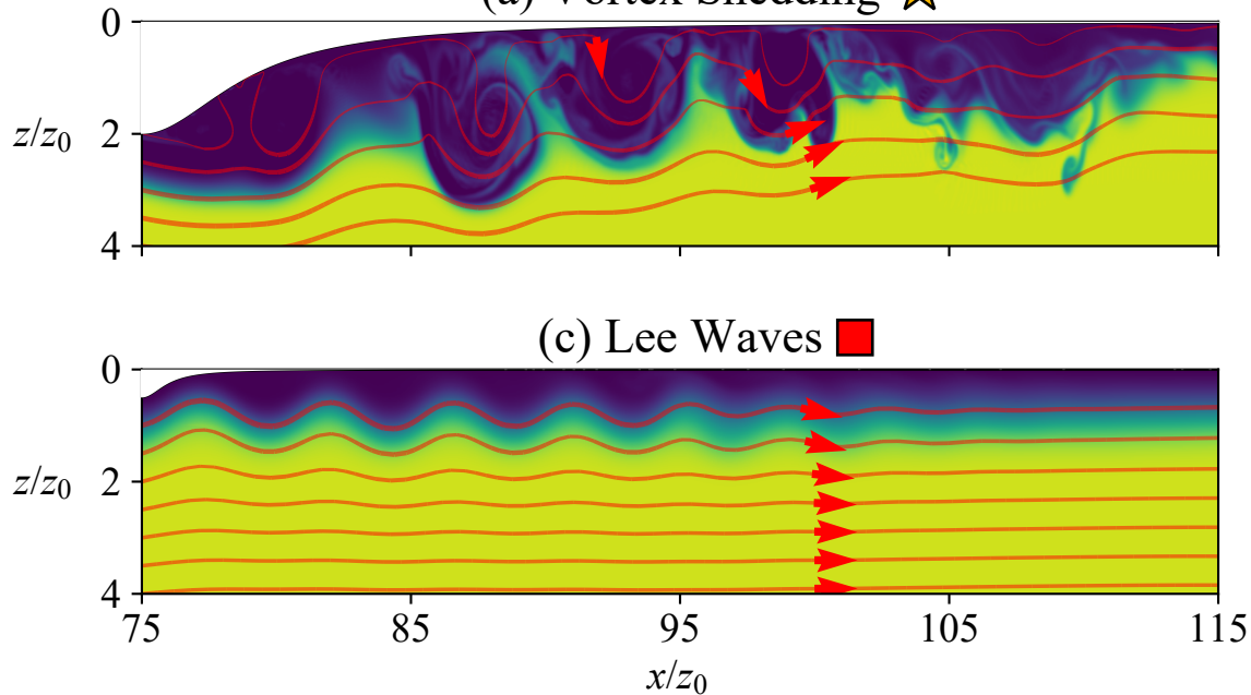
(a) Vortex Shedding ☆
