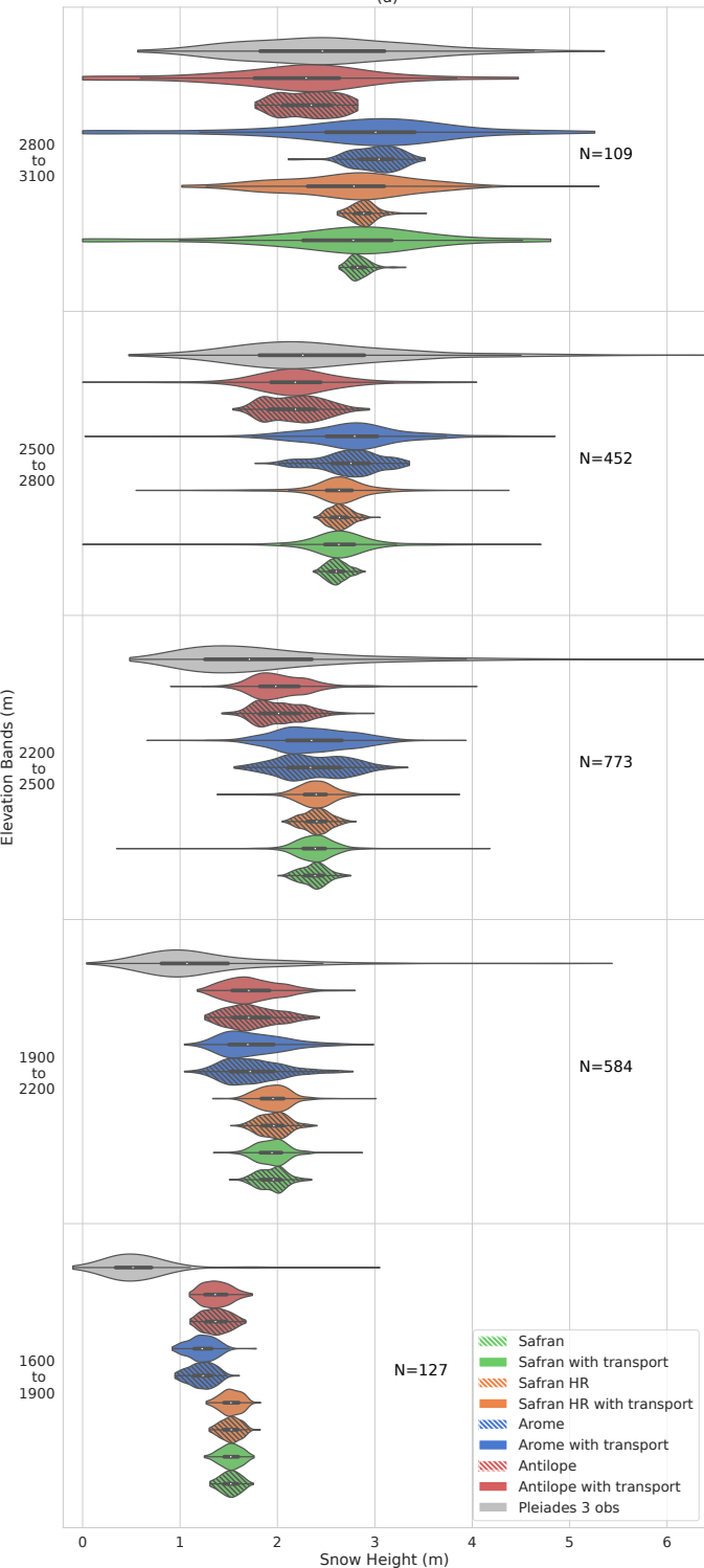
Pleiades 3 Galibier region January 23 2018 (a)
