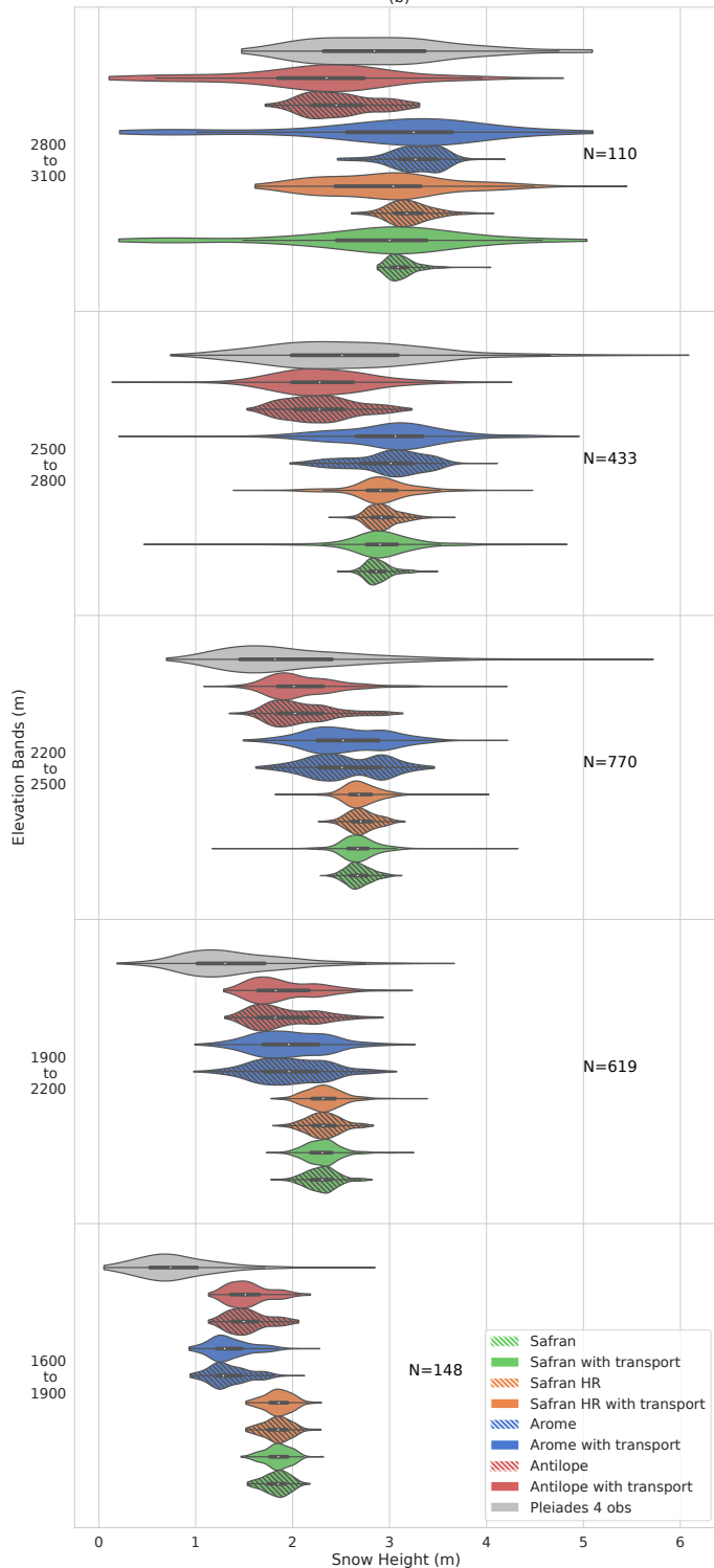
Pleiades 4 Galibier region March 16 2018 (b)
