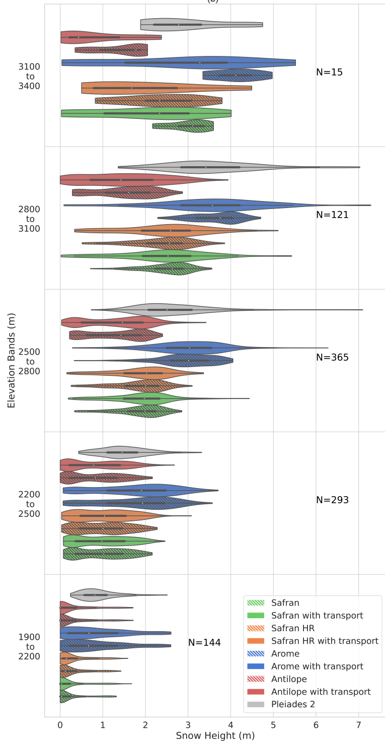
Pleiades 2 Grandes Rousses region 4 May 2020 (b)
