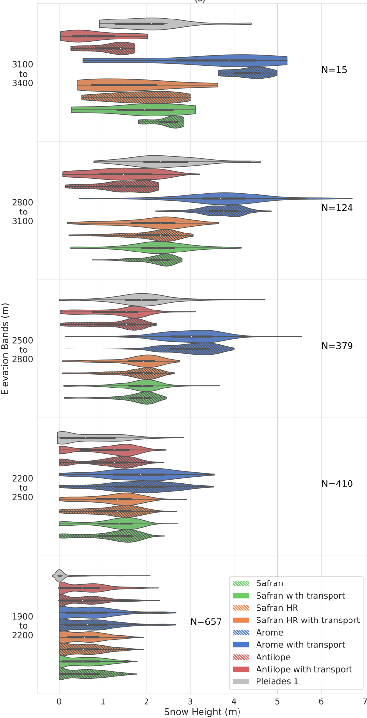
Pleiades 1 Grandes Rousses region 13 May 2019 (a)
