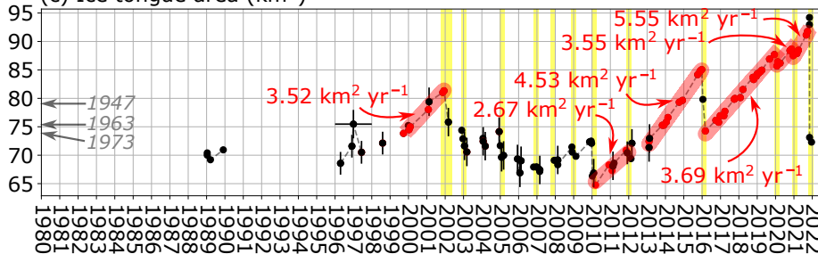
(c) Ice tongue area ( \text{km}^2 )
