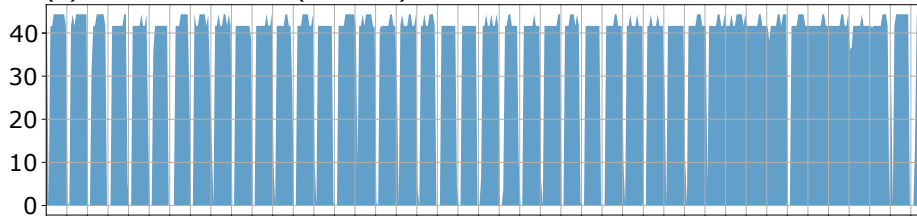
(b) Sea Ice Concentration (%) - Days with SIC < 15 %
