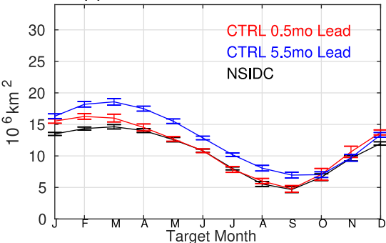
(b) Arctic SIV: Mean and STD
