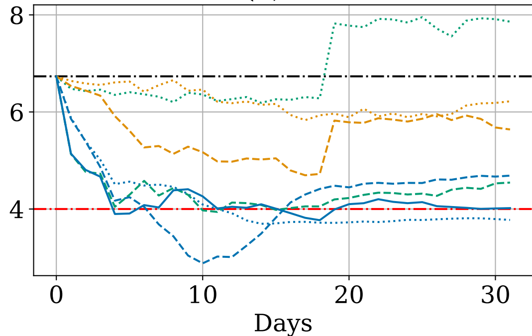
(a) \alpha
