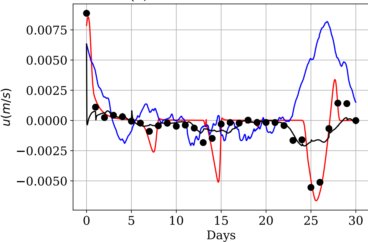
(c) u from SIC+SIT+SIV
