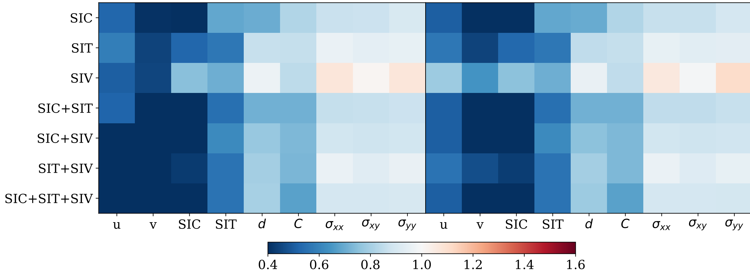
(a) \text{RMSE}^a/\text{RMSE}^{\text{free}}
