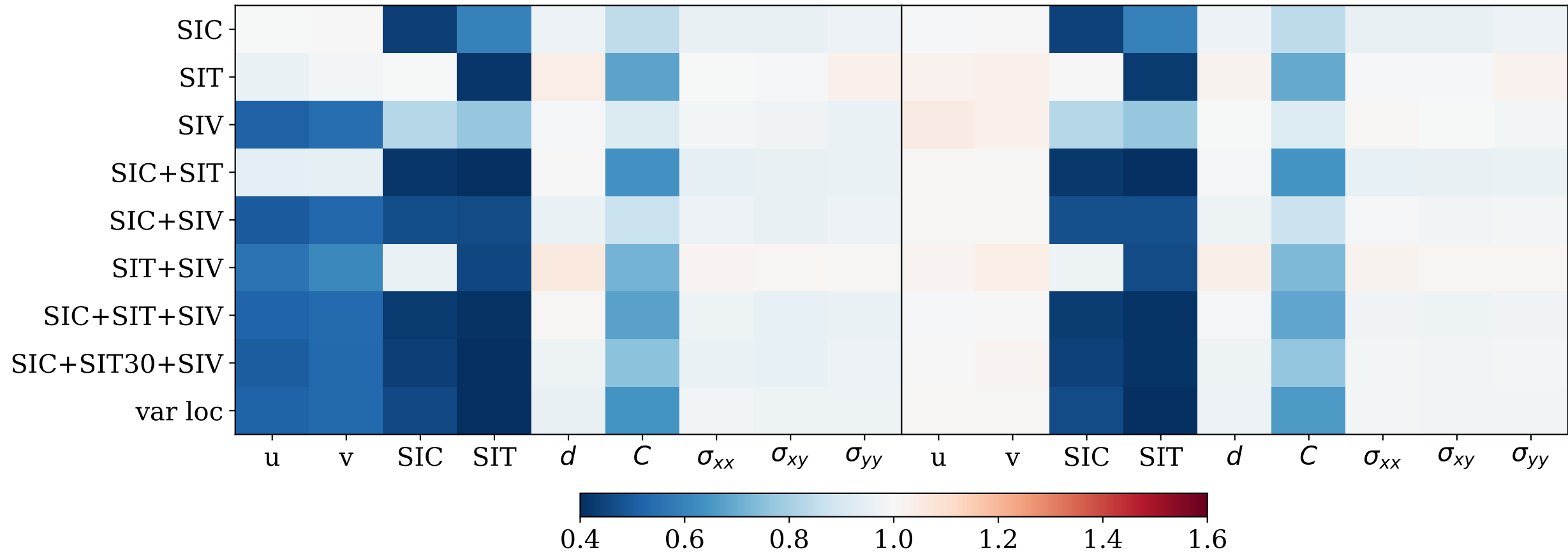
(a) \text{RMSE}^a/\text{RMSE}^{\text{free}}
