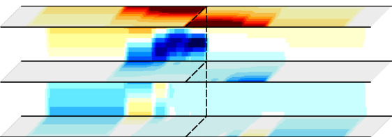
(b) Sum of Kelvin waves
