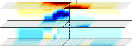
(c) MITgcm simulation Vorticity advection Poincaré waves
