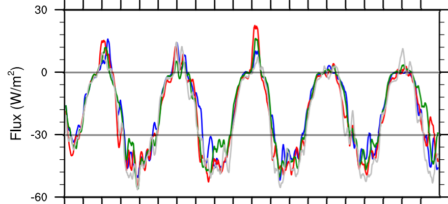
(a) Ice-atmosphere heat flux
