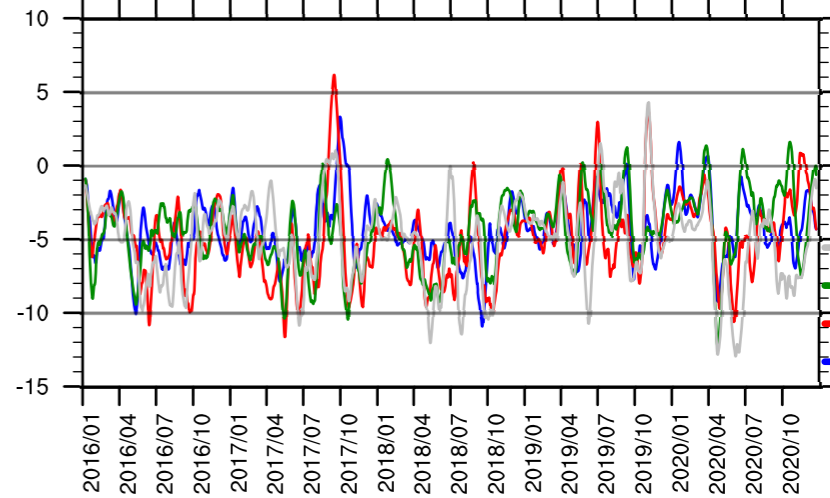
(f) Latent heat flux
