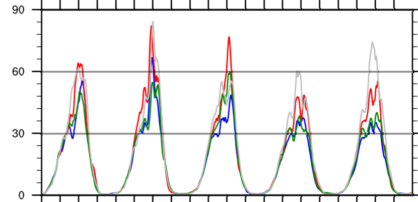
(c) Net shortwave flux
