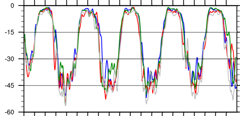
(b) Conductive heat flux at ice top layer
