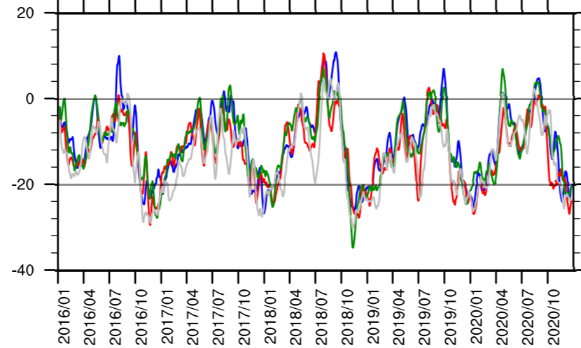
(e) Sensible heat flux
