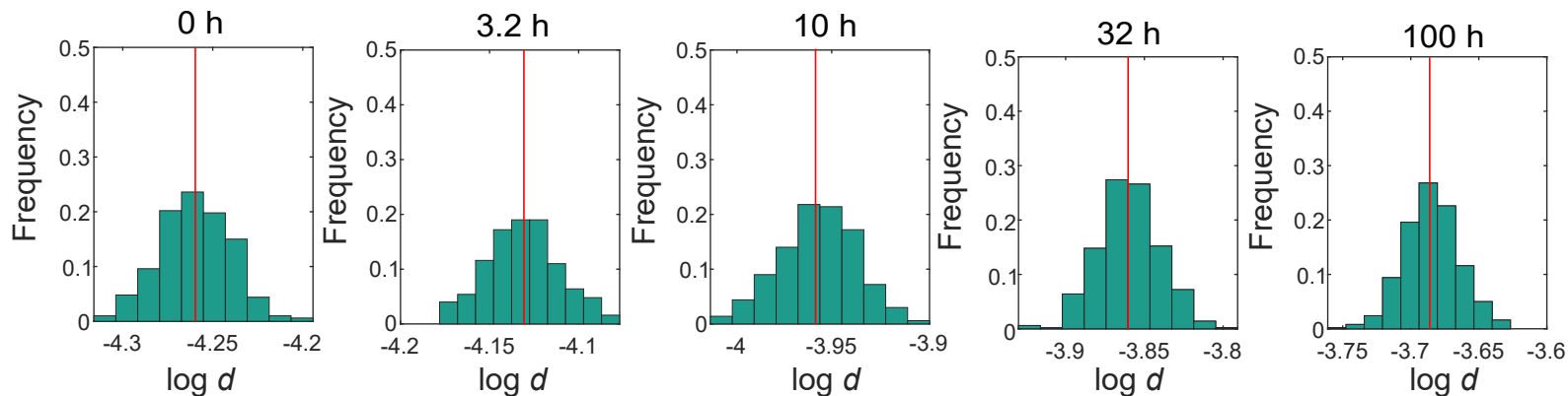
(a) 500 sets of variation-added grain size distribution for each duration
