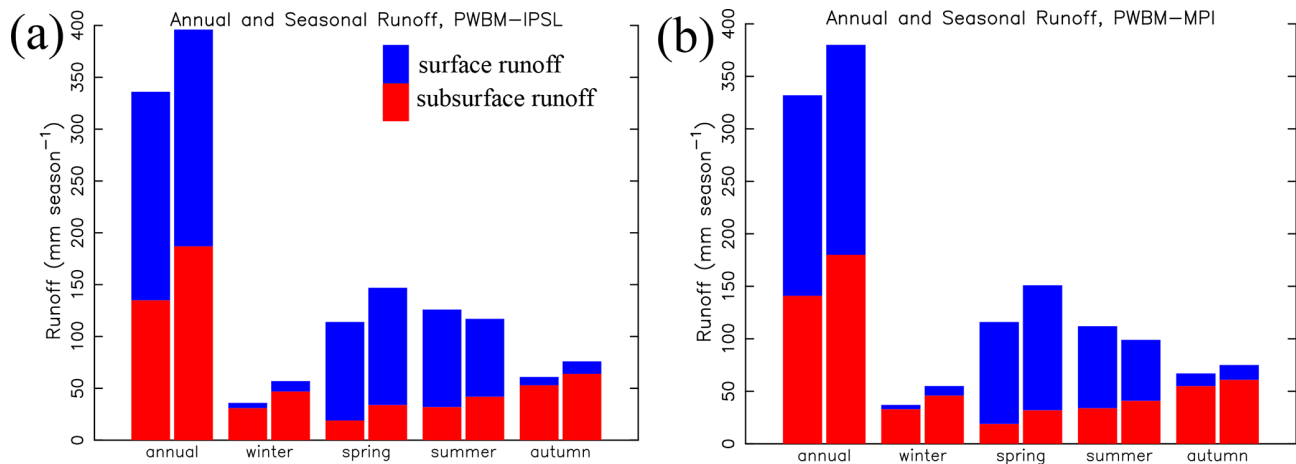
Figure 10. Annual and seasonal total runoff for the early-century (left bar for each period) and late-century (right bar for each period) periods, expressed as surface (blue) and subsurface (red) amounts for (a) PWBM-IPSL and (b) PWBM-MPI simulations.
